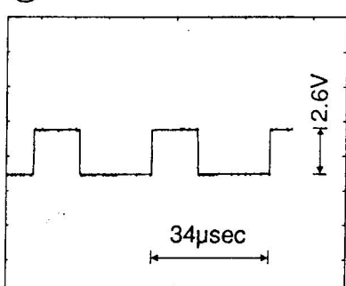
⑫ IC400 Pin11
