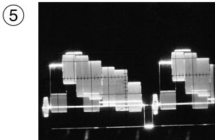
IC301 Pin 26 500mV/10msec DIV VV/EE (VIDEO OUT)
