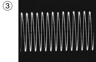
IC301 Pin 41 100mV/0.2msec DIV REC/PB (2fsc)
