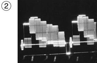
IC301 Pin 32 200mV/10msec DIV EE (VIDEO IN)
