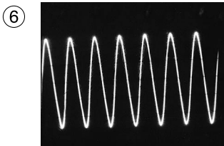
IC301 Pin 49 100mV/0.2msec DIV PB/REC (3.58MHz X-TAL IN)
