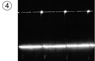
IC301 Pin 25 1.0V/20msec DIV VV/EE (C-SYNC OUT)
