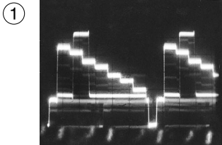
IC301 Pins 20, 21, 22 100mV/10msec DIV VV/EE 20 Main DE Emphasis Filter 21 Main DE Emphasis out 22 Clamp in
