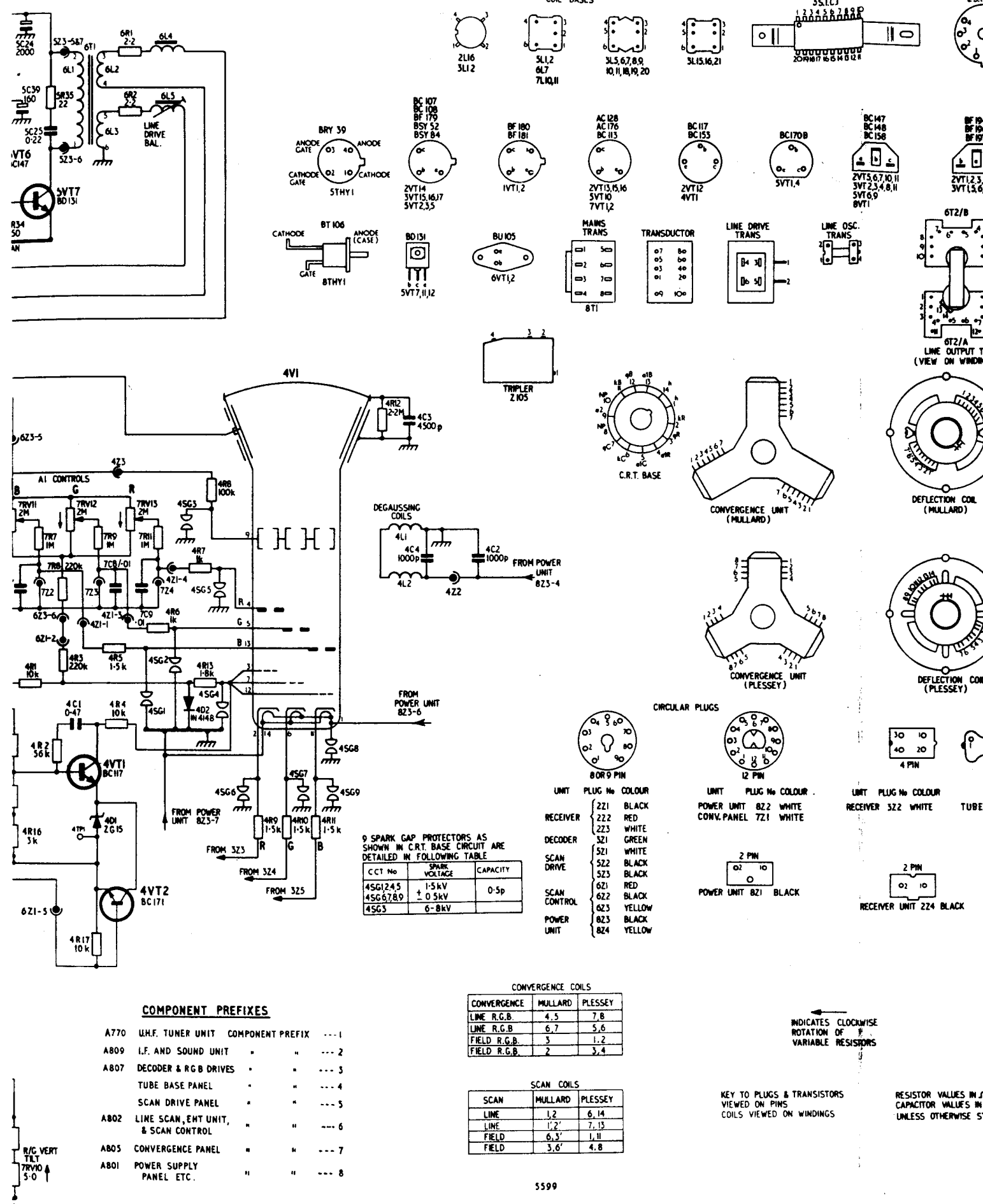
TIMEBASE, E.H.T. & CONVERGENCE CIRCUITS DIAGRAM
