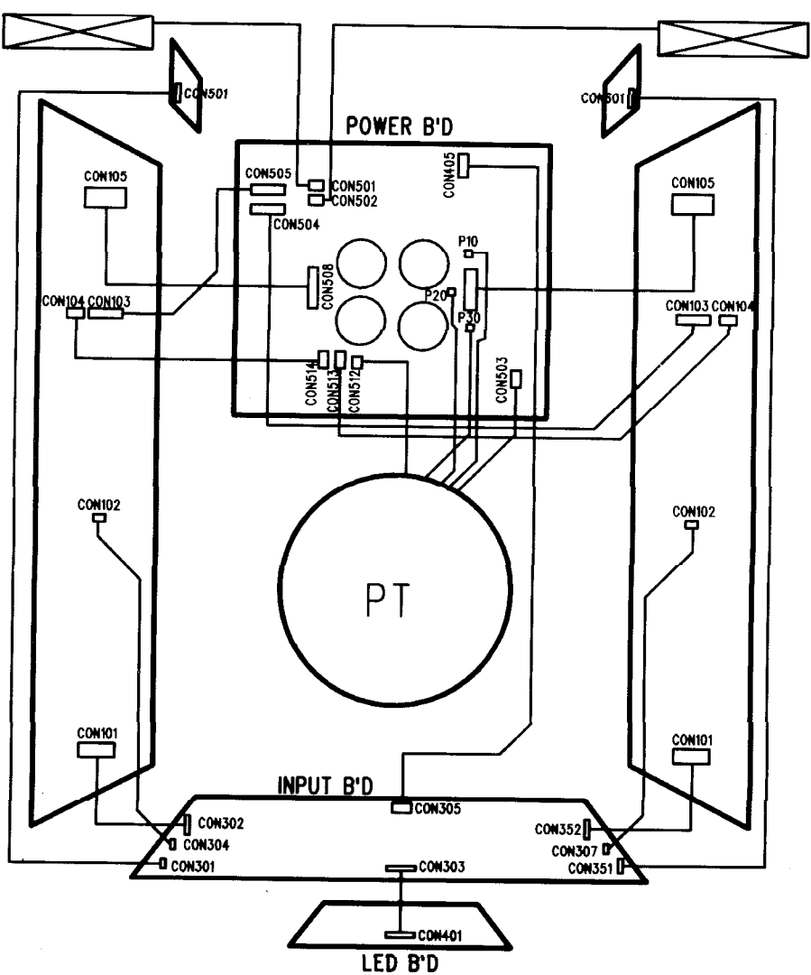
Wiring Diagram (MA-630/930)
