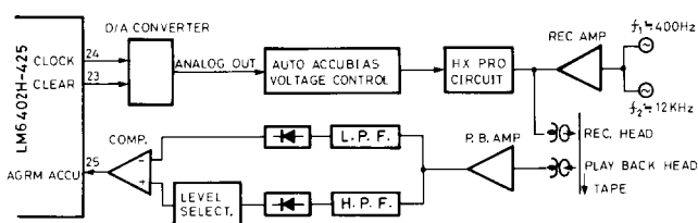
Fig. 1 Block diagram
