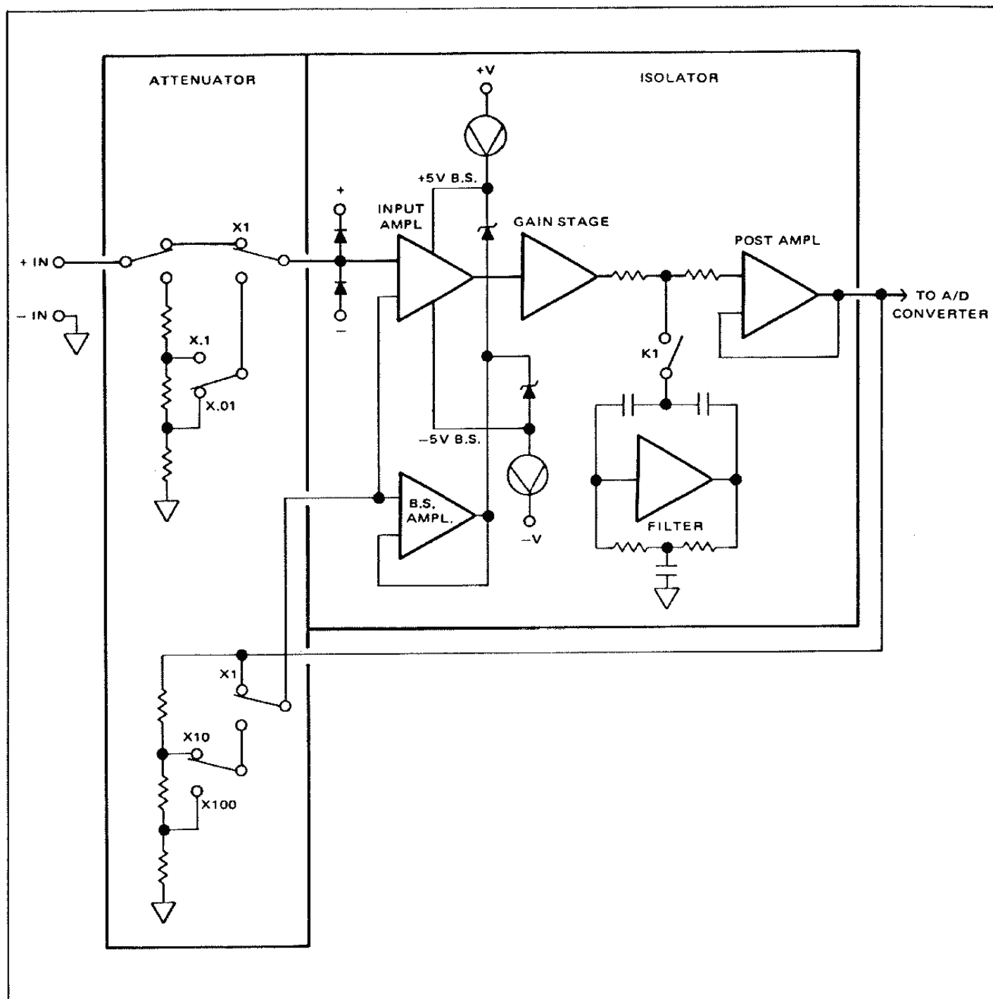
Figure 4.10 - Attenuator/Isolator DC
