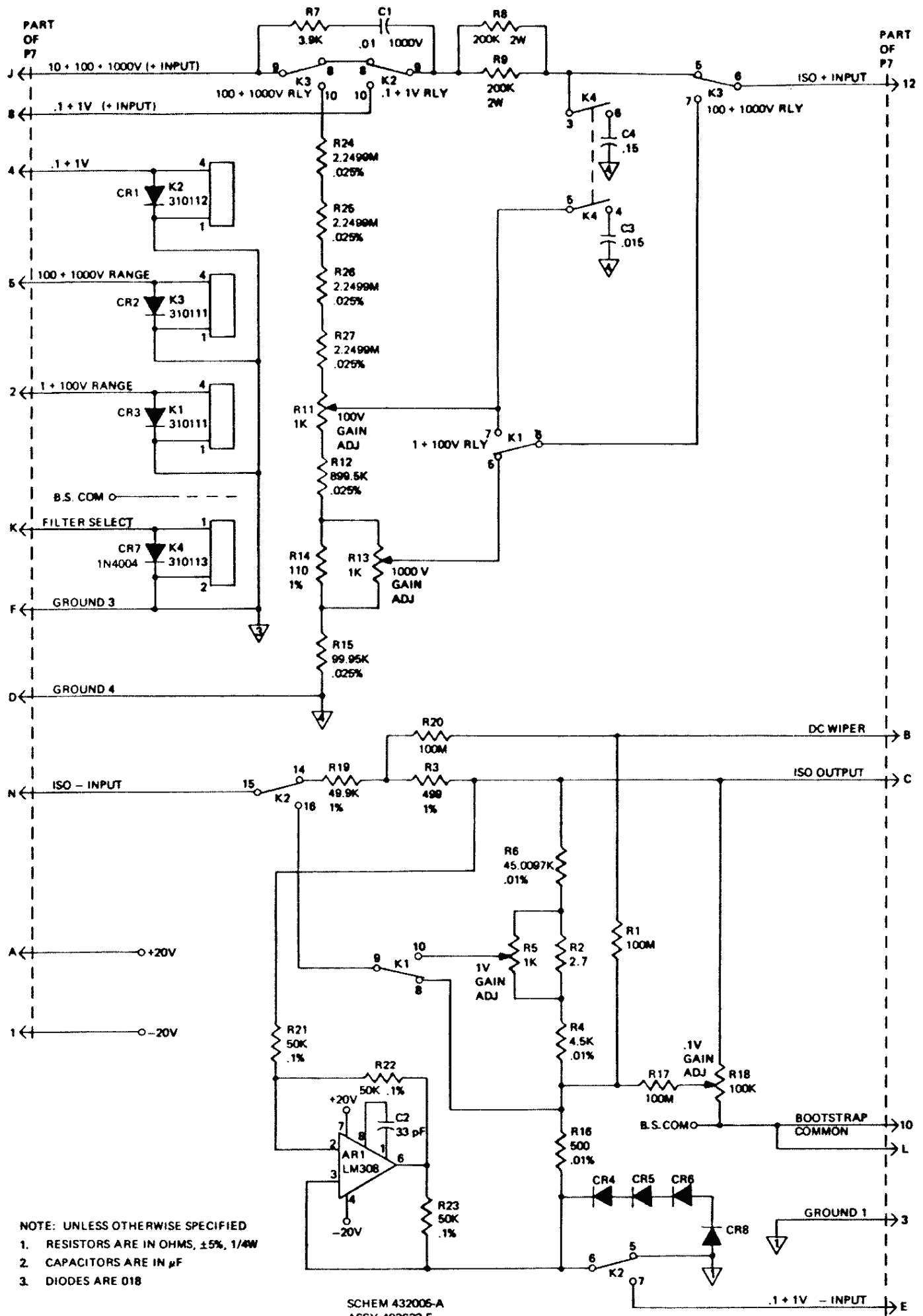
Figure 6.6 - Schematic, Attenuator
