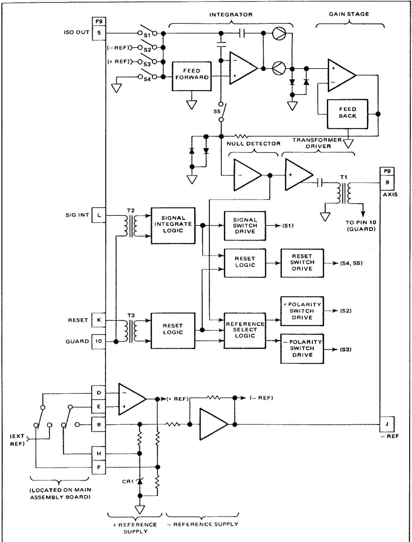
Figure 4.12 - Digitizer
