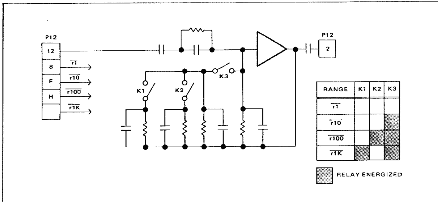
Figure 4.7 - Scaling Amplifier
