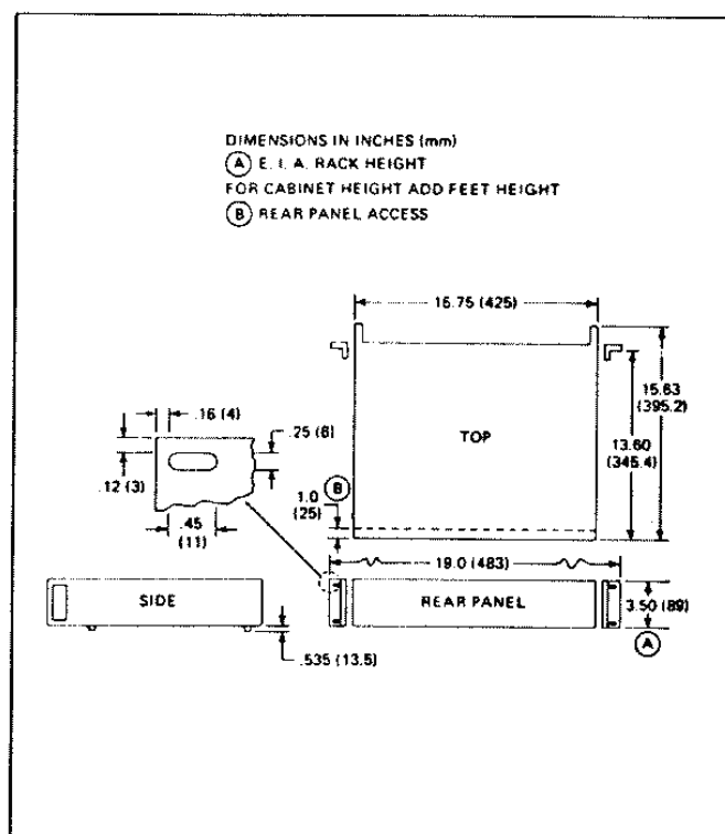
Figure 1.2 - Dimensions
