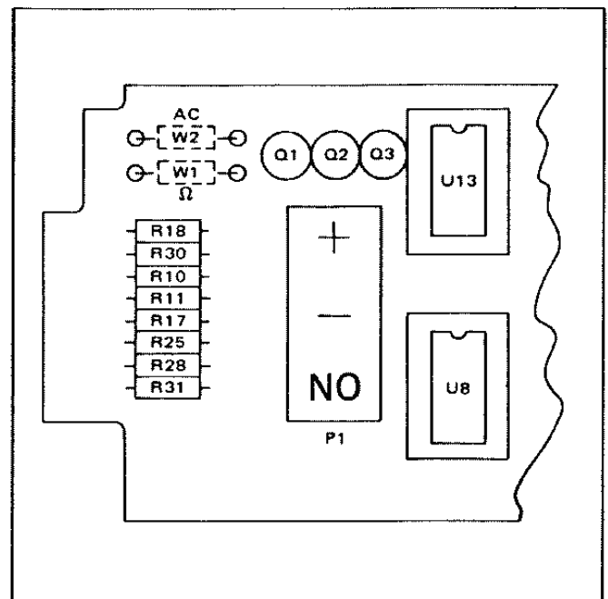
Figure 2.17 - Jumper Location
