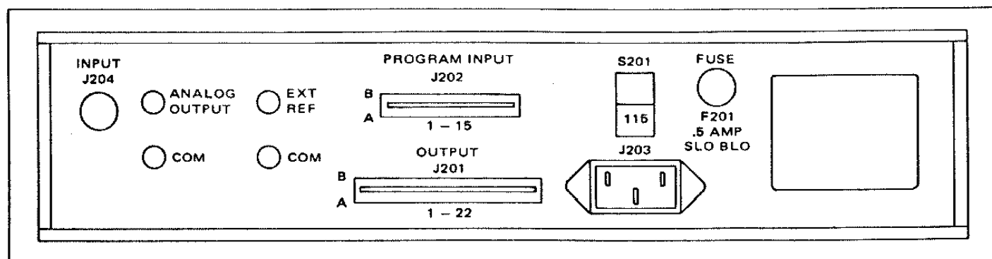
Figure 2.10 - Rear Panel
