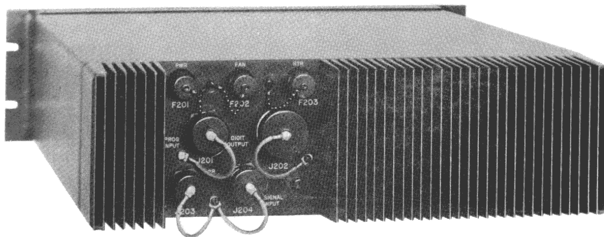
(b) Rear Panel Connectors
