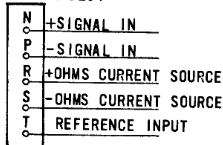
Figure 2.2. Input Connector
