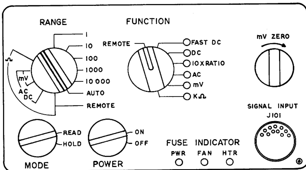
Figure 2.1. Control Panel
