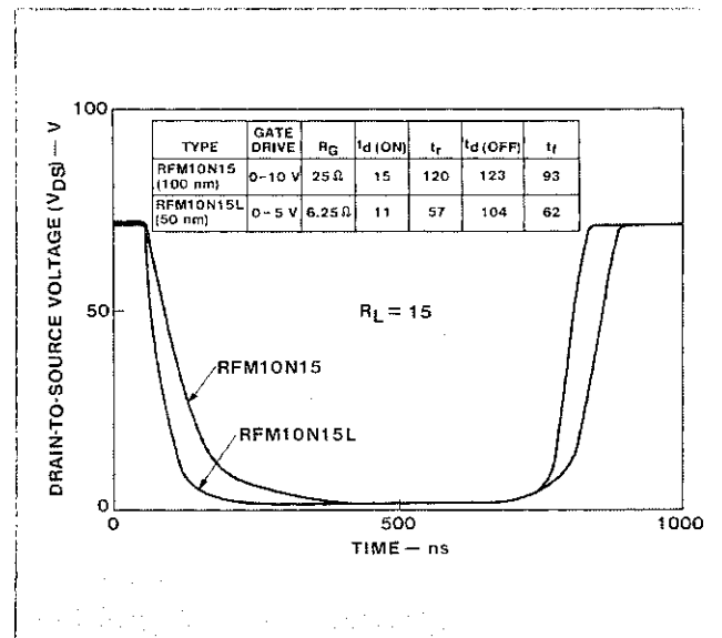
Drain voltage turn-on waveforms for L 2 FETs and standard MOSFETs.
