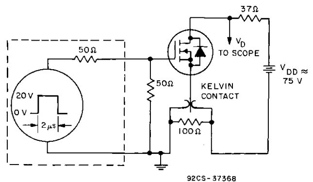
Fig. 11 - Switching Time Test Circuit.
