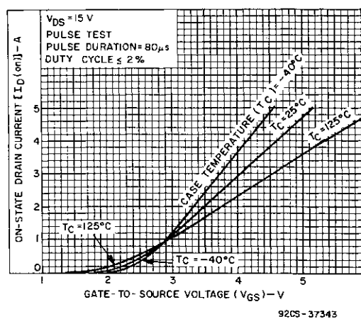
Fig. 5 — Typical transfer characteristics for all types.
