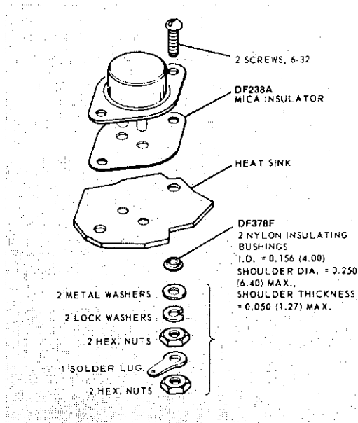
Suggested mounting hardware for JEDEC TO-204AE
