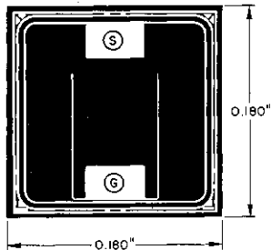
⑤ SOURCE ATTACH AREA 0.030" x 0.060" ⑥ GATE ATTACH AREA 0.030" x 0.060" BACK SIDE — DRAIN
