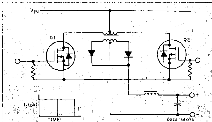
Push-Pull Converter
