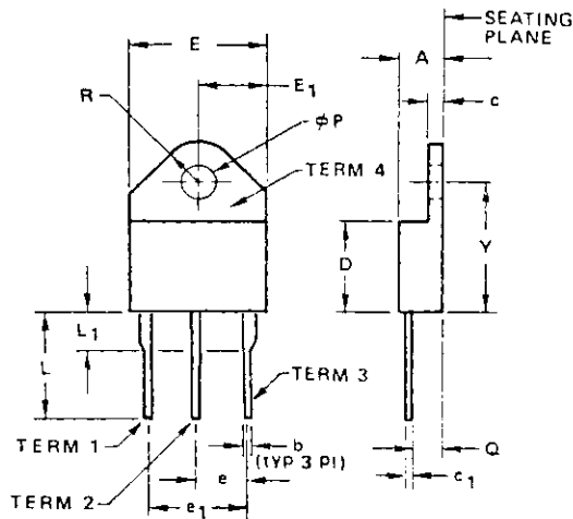
TO-218AC
