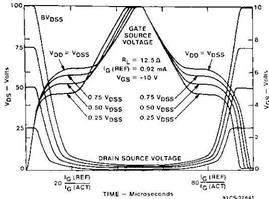
Fig. 6 - Normalized switching waveforms for constant gate-current drive.
