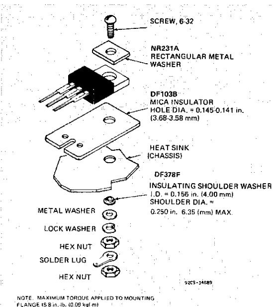
Suggested mounting hardware for JEDEC TO-220AB.
