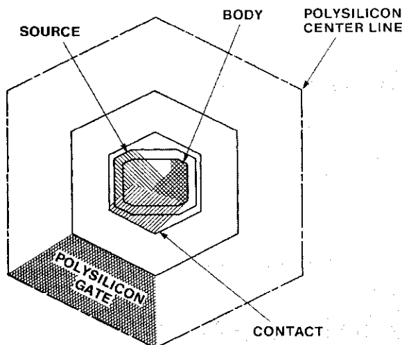
Hexagonal unit cell used in RCA power MOSFET chips.
