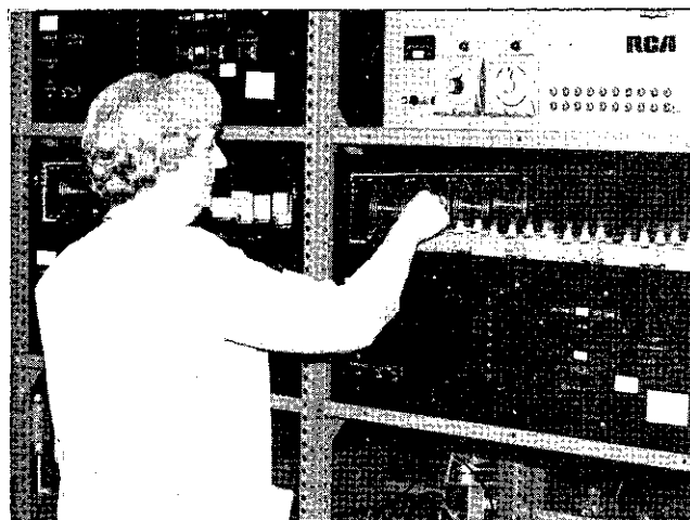
Thermal-fatigue and operating-life test racks.
