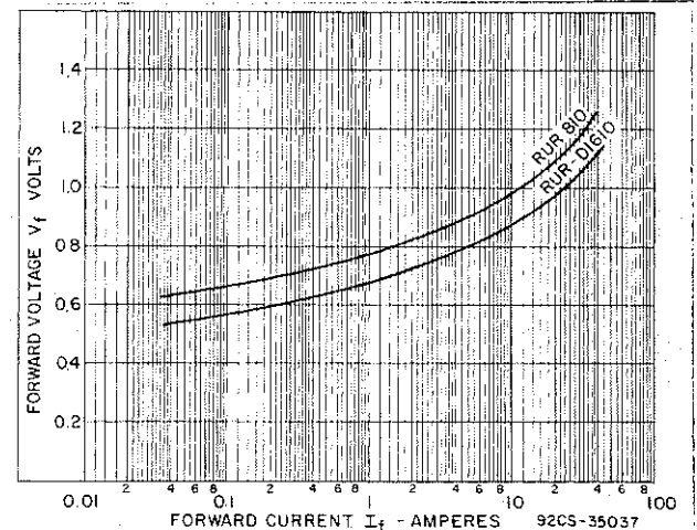
Maximum forward voltage as a function of forward current.
