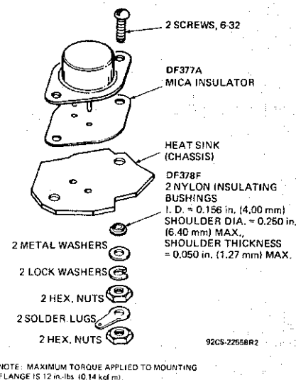
Suggested mounting hardware for JEDEC TO-204MA (Formerly JEDEC TO-3).
