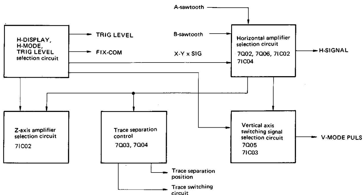
Figure 2-5-1. Horizontal control circuit 6 , 7
