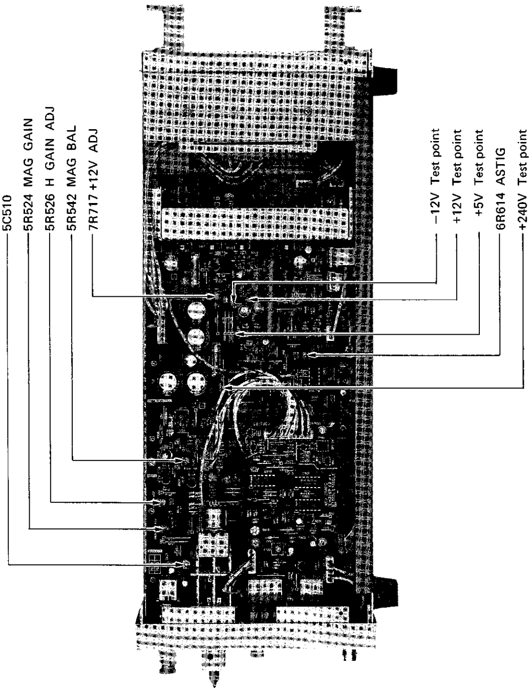
Figure 4-7-1-2: Right-Side View SS-5702A/5703A
