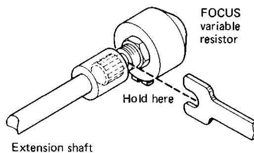
Junction between FOCUS variable resistor and extension shaft
