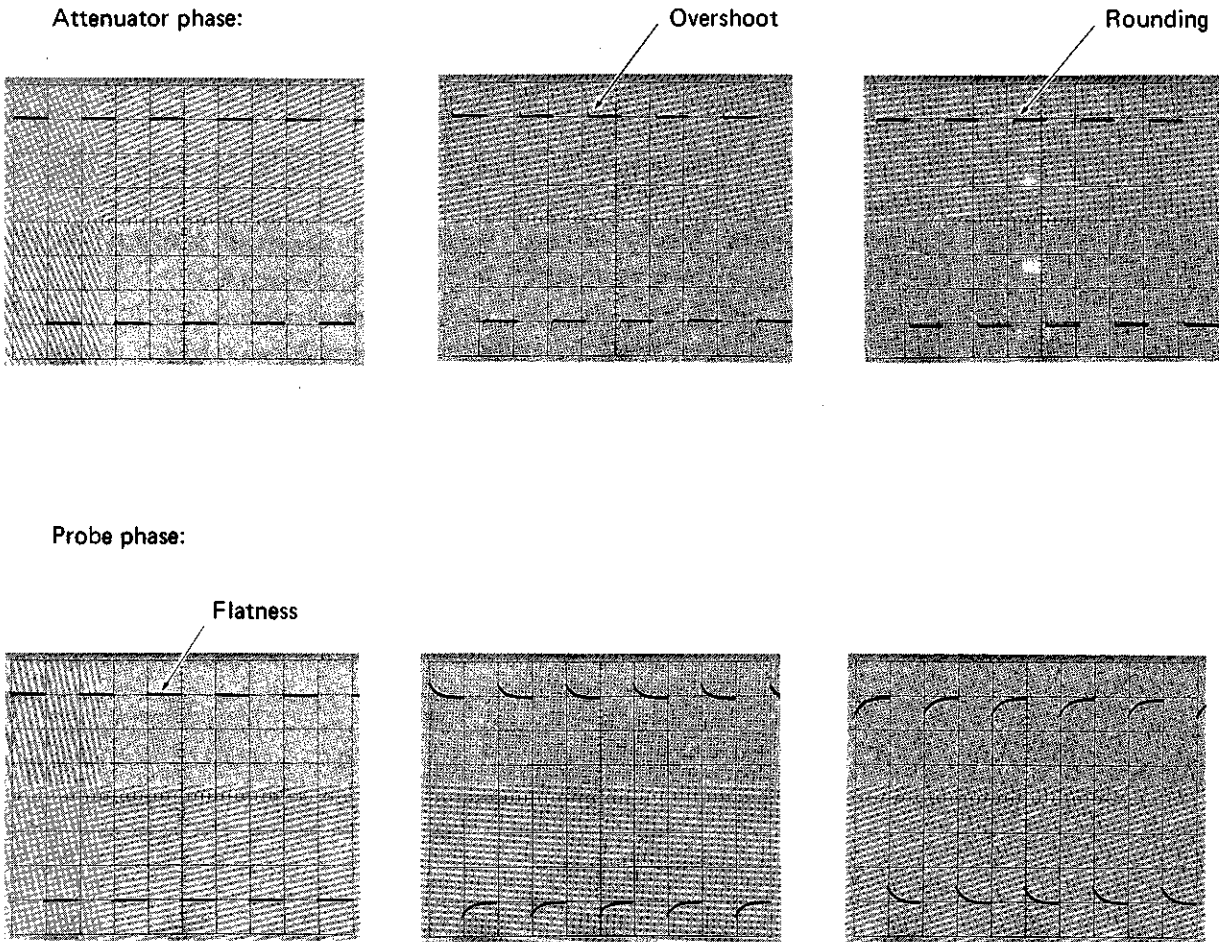
Figure 4-7-4 Phase Waveforms
