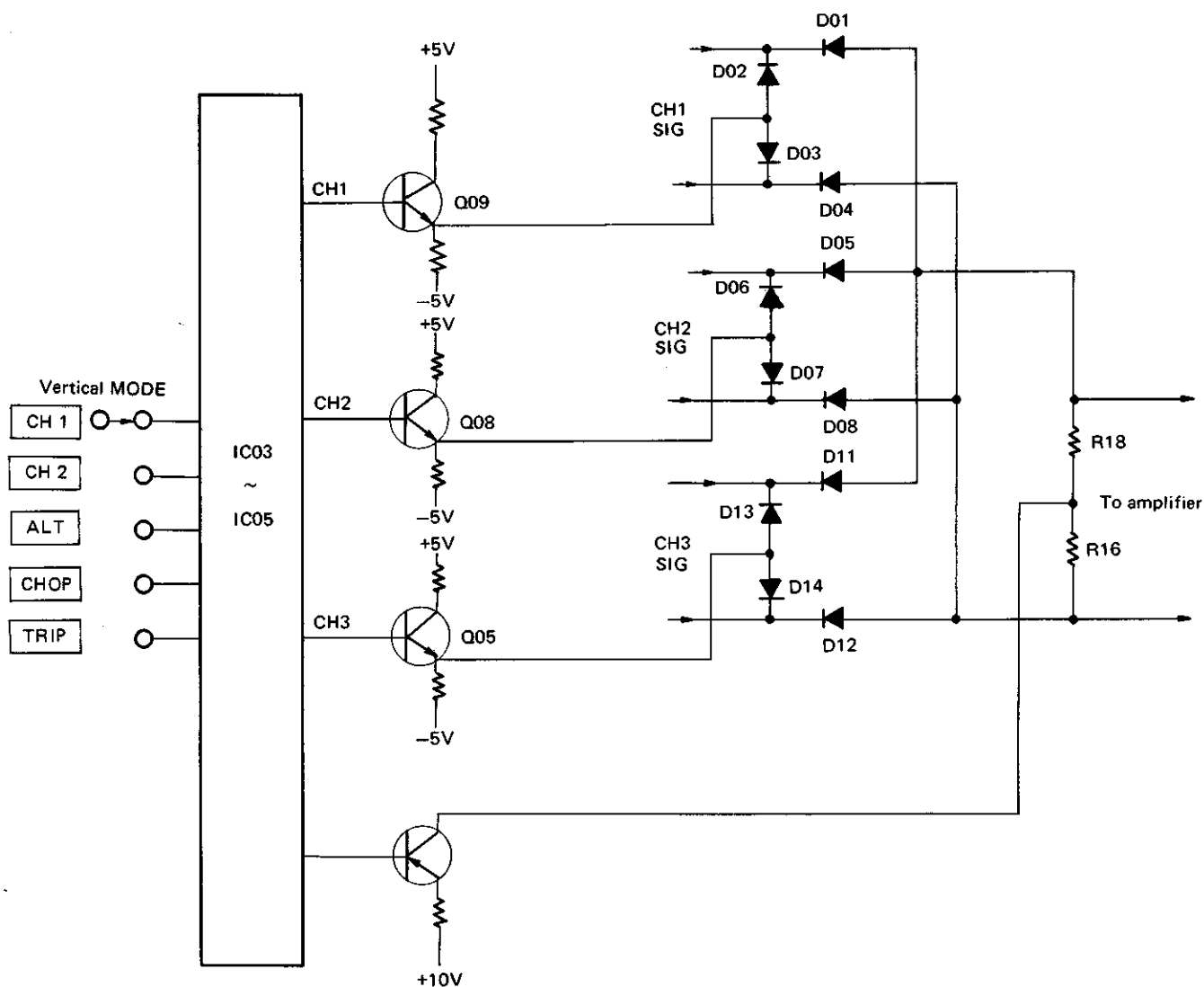
Figure 2-2-5. Switching circuit 3
