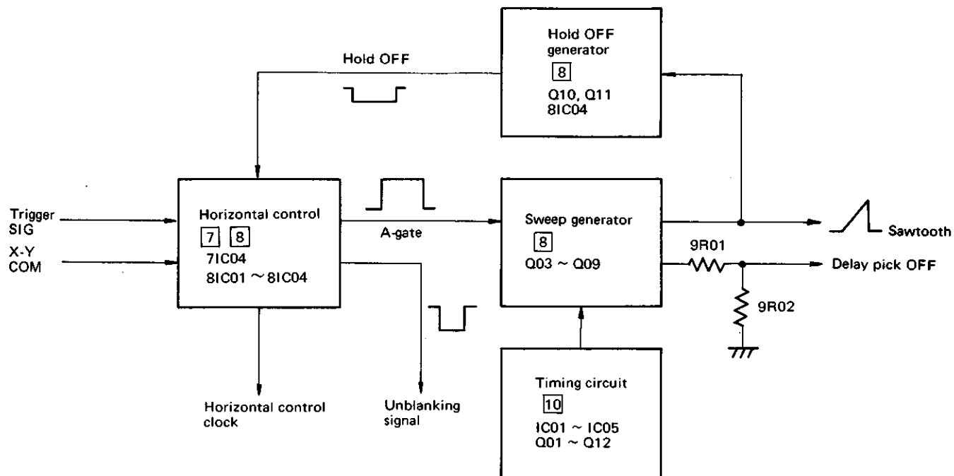
Figure 2-4-1-(1) A-sweep signal generation circuit [7], [9]
