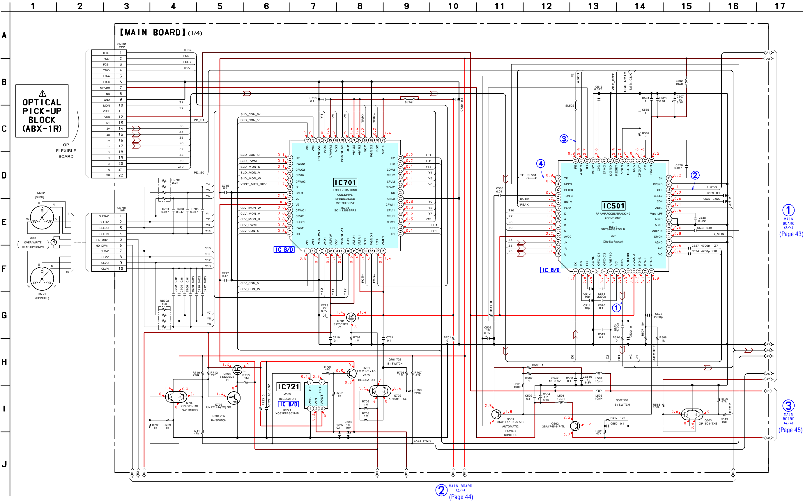
6-6. SCHEMATIC DIAGRAM – MAIN Board (1/4) – • See page 39 for Waveforms. • See page 46 for IC Block Diagrams.
