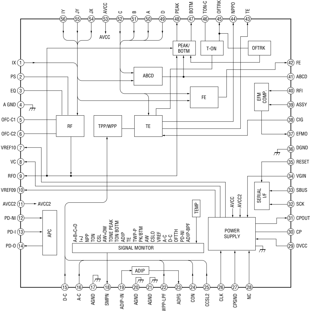
IC501 SN761058AZQLR
