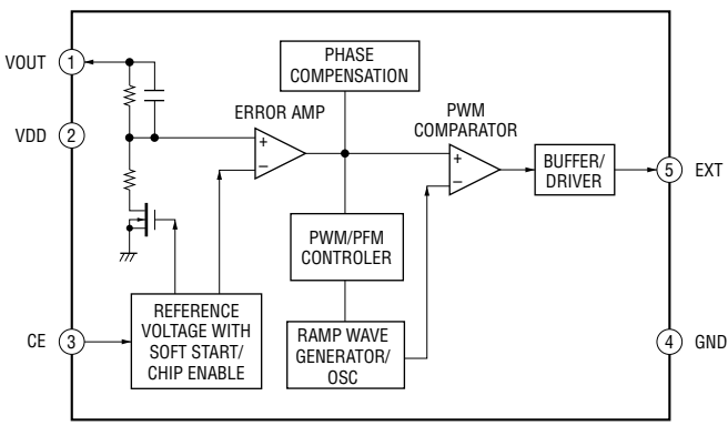
IC651 XC6367A331MR
