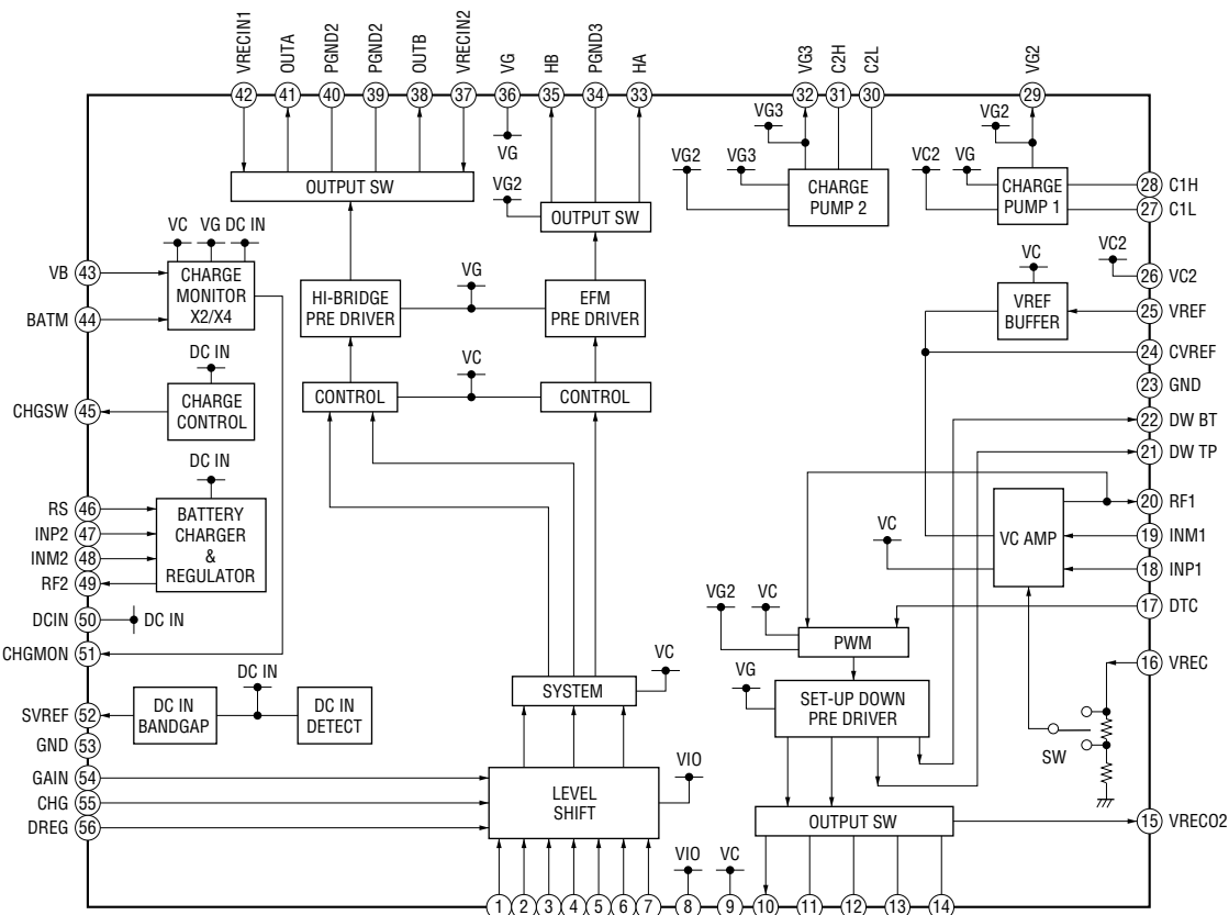
IC601 XPC18A22AEPR2
