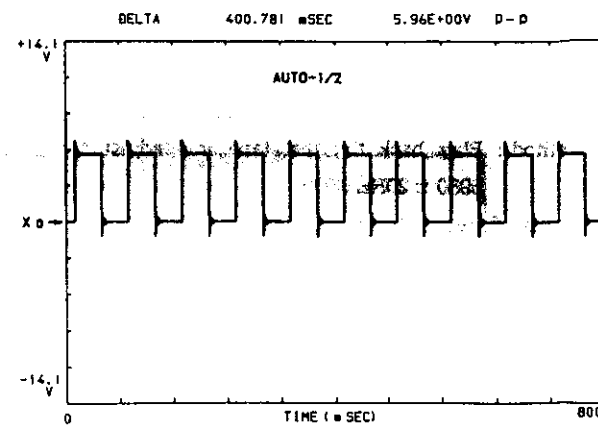
⑩ IC901 PIN ②①, ②②
