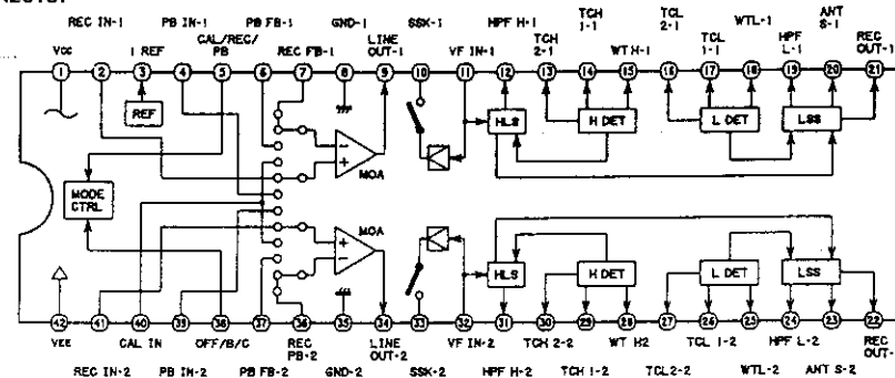
IC, CX20187
