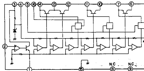
IC, LB1408
