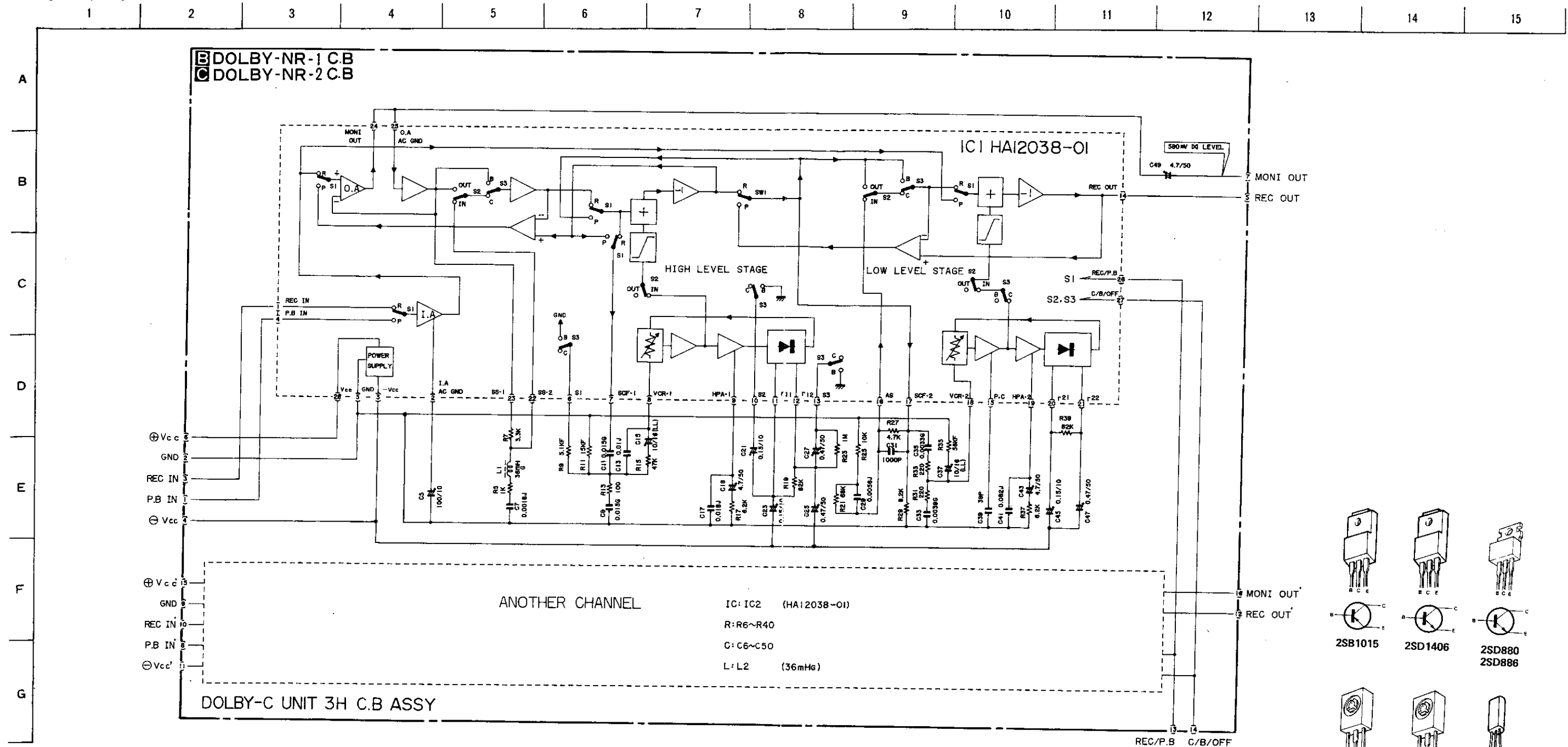
SCHEMATIC DIAGRAM-2
