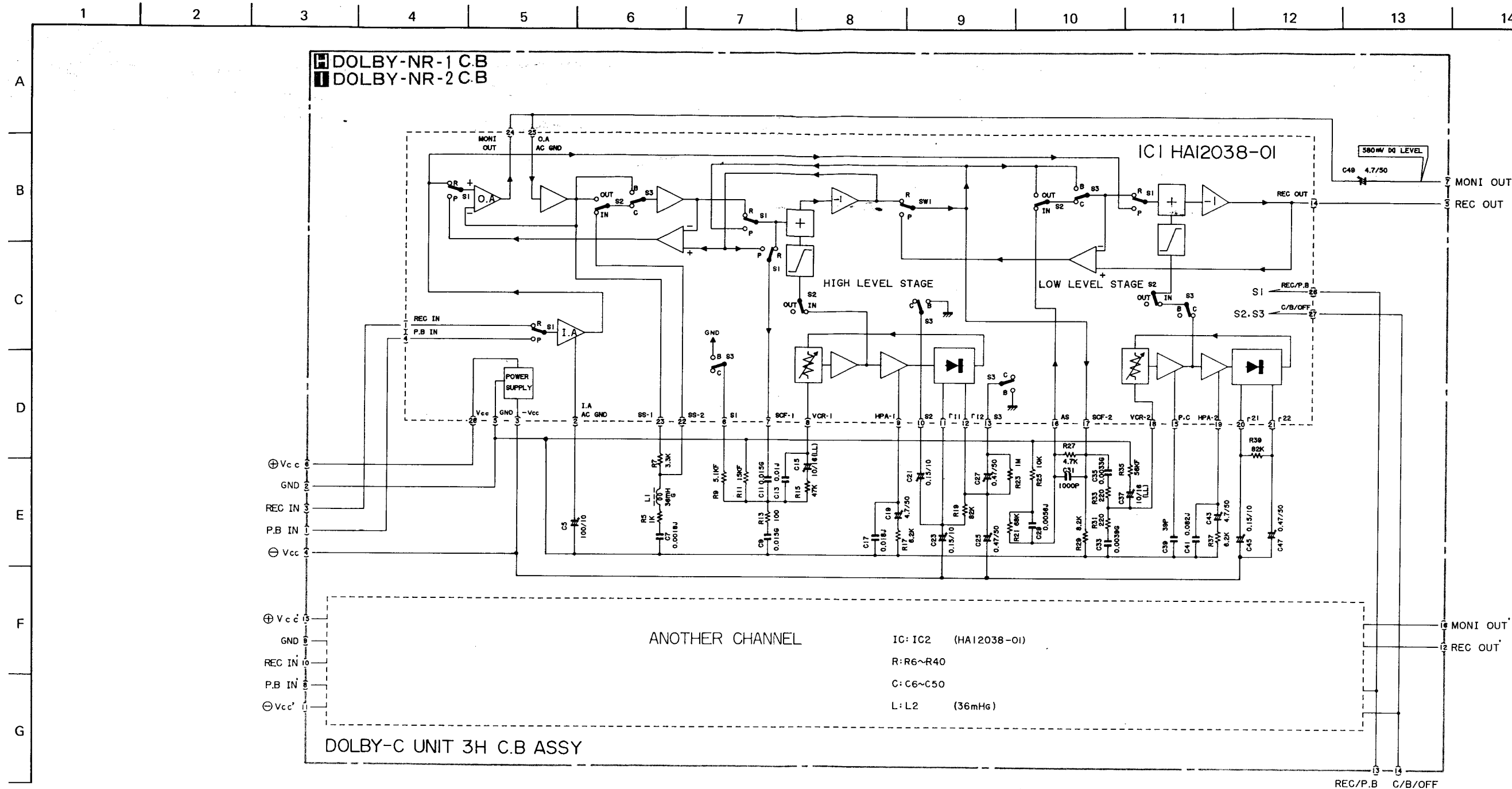
SCHEMATIC DIAGRAM-1
