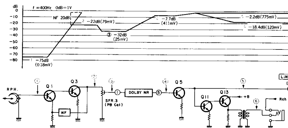
LEVEL DIAGRAM
