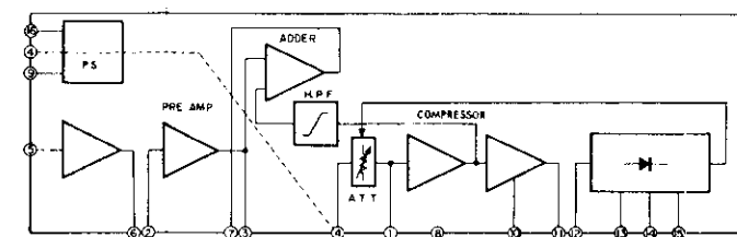
IC BLOCK DIAGRAM NE545B
