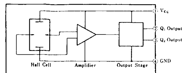
IC BLOCK DIAGRAM NE545B
