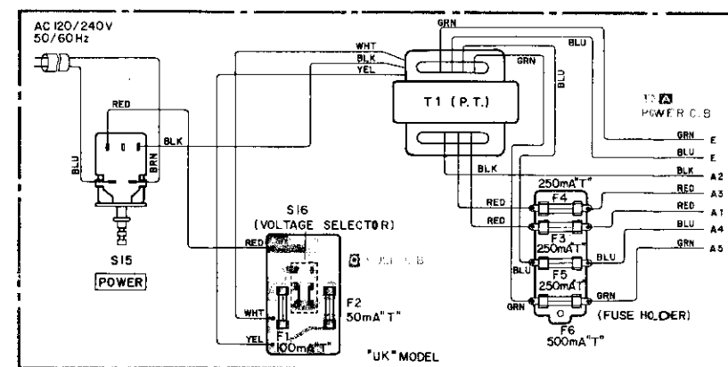
POWER CIRCUIT BOARD
