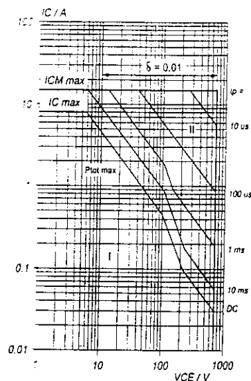
Fig. 12 Forward bias safe operating area. T_{Hs} = 25\text{ }^{\circ}\text{C} I Region of permissible DC operation II Extension for repetitive pulse operation
