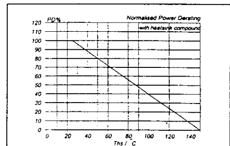
Fig. 8 Normalised power dissipation PD\% = 100 P_D/P_{D 25^{\circ}\text{C}} = f(T_{HS}) .
