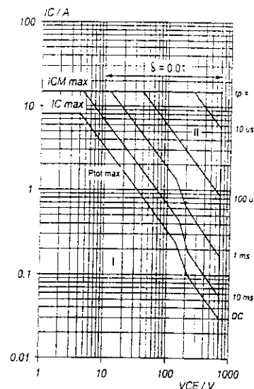
Fig. 13 Forward bias safe operating area. T_{Hs} = 25\text{ }^{\circ}\text{C} I Region of permissible DC operation II Extension for repetitive pulse operation
