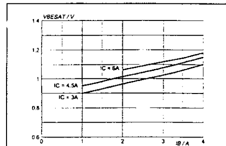
Fig. 6 Typical base-emitter saturation voltage. V_{BEsat} = f(I_B) ; parameter I_C
