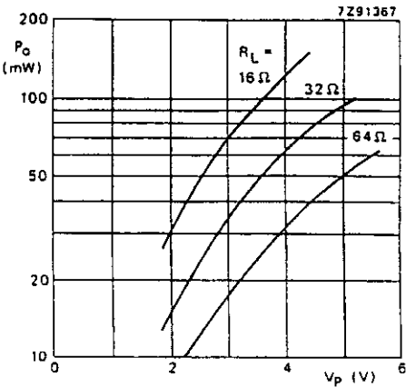
Fig. 3 Output power across the load impedance ( R_L ) as a function of supply voltage ( V_p ) in stereo application. Measurements were made at f = 1\text{ kHz} ; d_{tot} = 10\% ; T_{amb} = 25^\circ\text{C}
