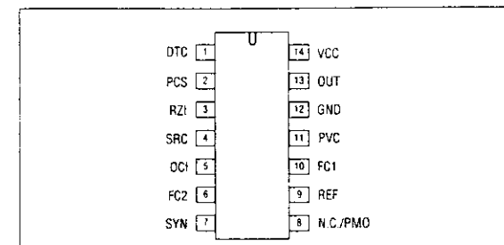
Pin Configuration (top view)
