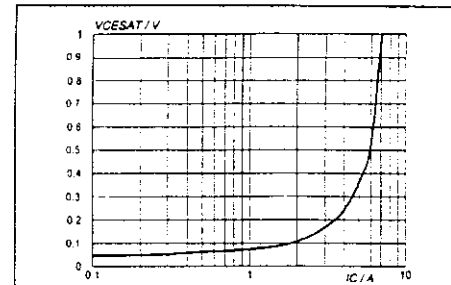
Fig. 5 Typical collector-emitter saturation voltage. V_{CEsat} = f(I_C) ; parameter I_B/I_C
