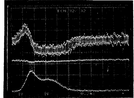
Waveform showing Short Kick Gain
