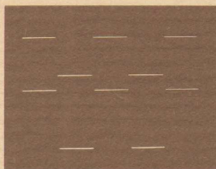
2 KHz Square Wave 150 Watts 8 Ohm Scope: 0.1 msec/cm Top: Input 1.0 v/cm Bottom: Output 20 v/cm
