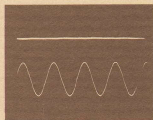
Sine Wave & Distortion Products 20 KHz 100 m Watt Scope: 20 \mu sec/cm Top: Distortion Products 0.2 v/cm Bottom: Output 1 v/cm
