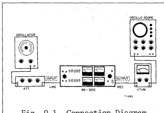
Fig. 9-1 Connection Diagram
