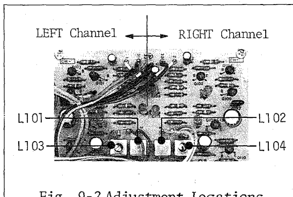
Fig. 9-2 Adjustment Locations
