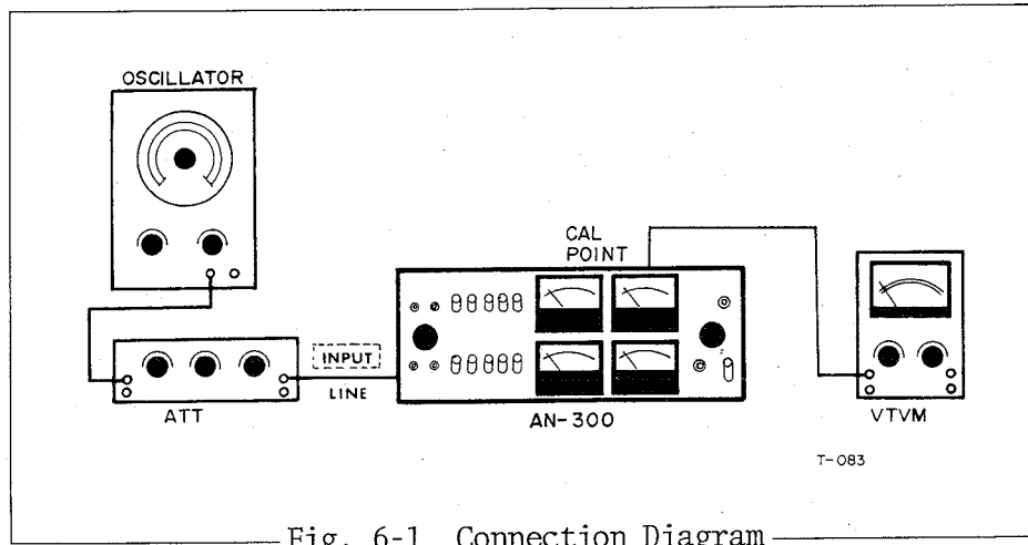
Fig. 6-1 Connection Diagram
