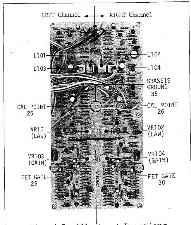
Fig. 6-3 Adjustment Locations
