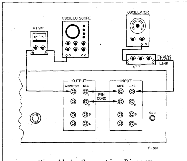
Fig. 11-1 Connection Diagram
