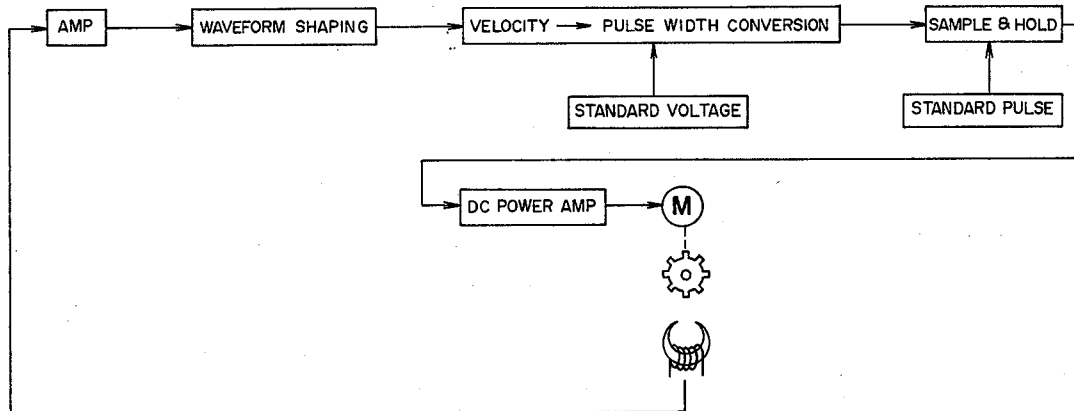
Fig. 5 Block Diagram
