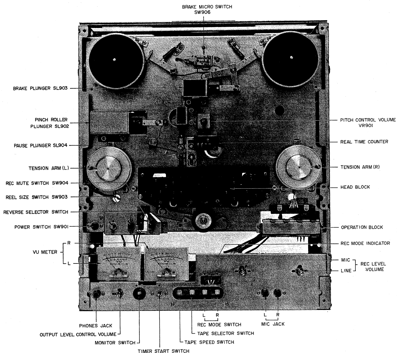
Fig. 2 Front View
