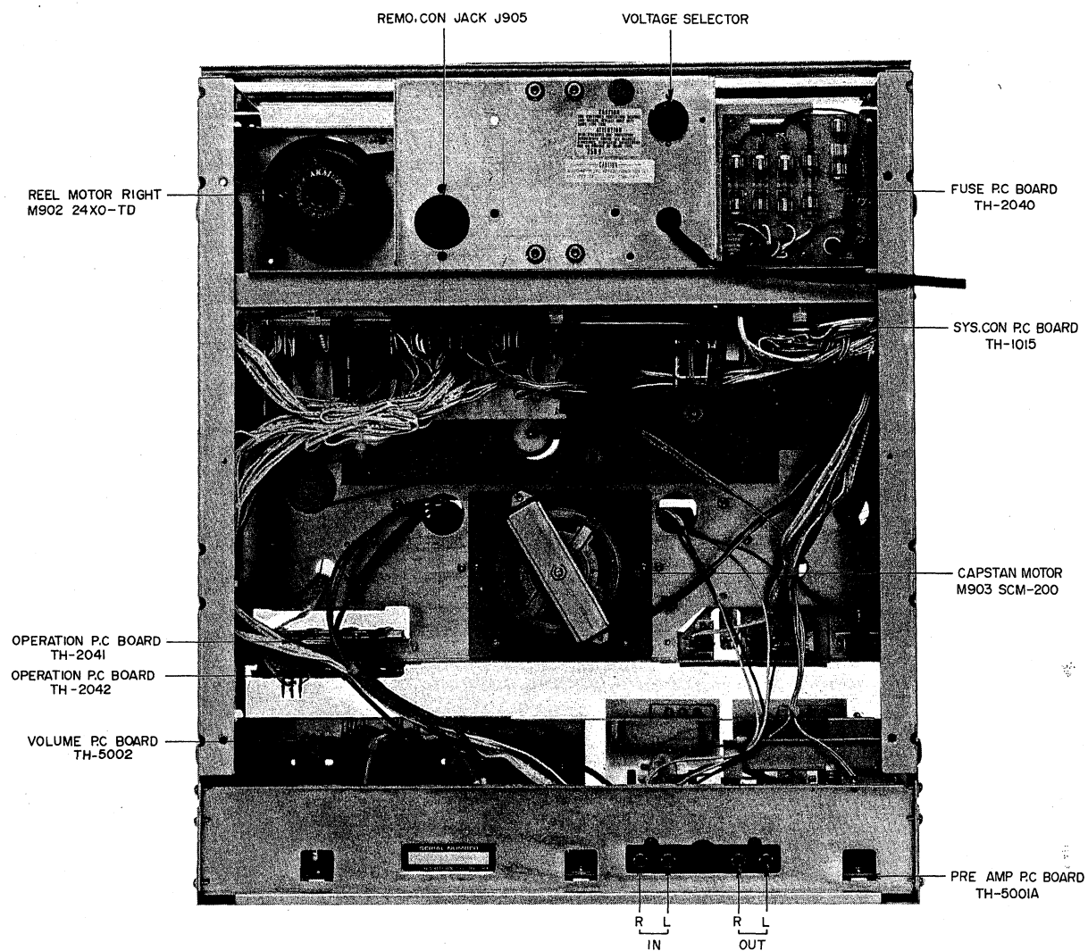
Fig. 3 Rear View
