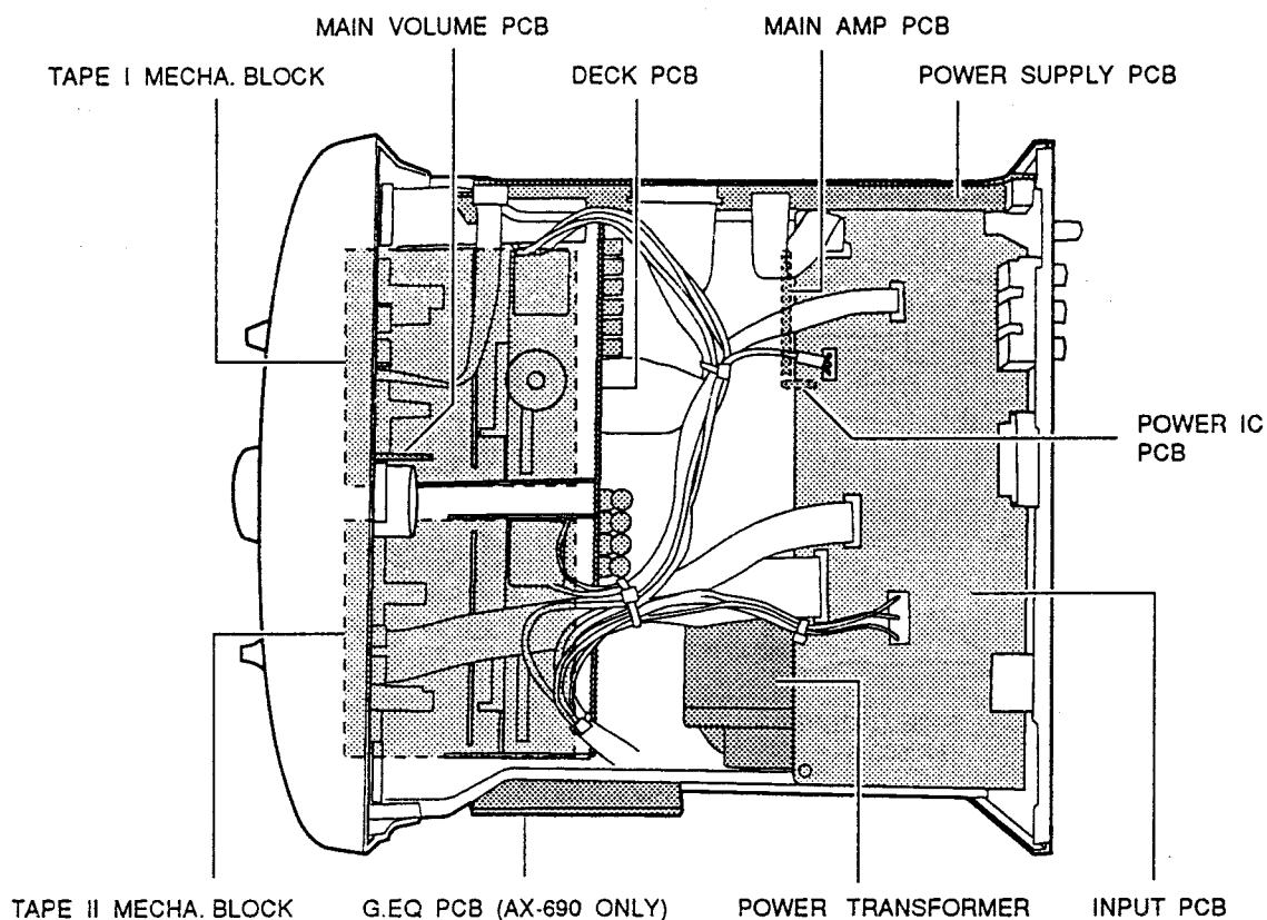
Fig. 2-1 Top view
