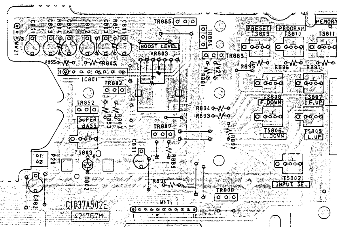
PRE AMP PCB C1037A502E (AX-690 ONLY)
