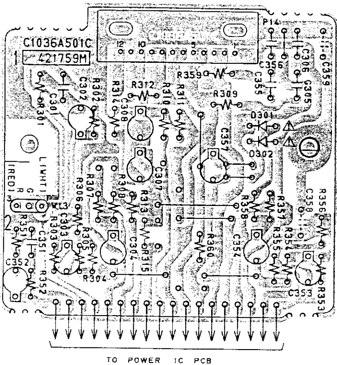
MAIN AMP PCB C1036A501C
