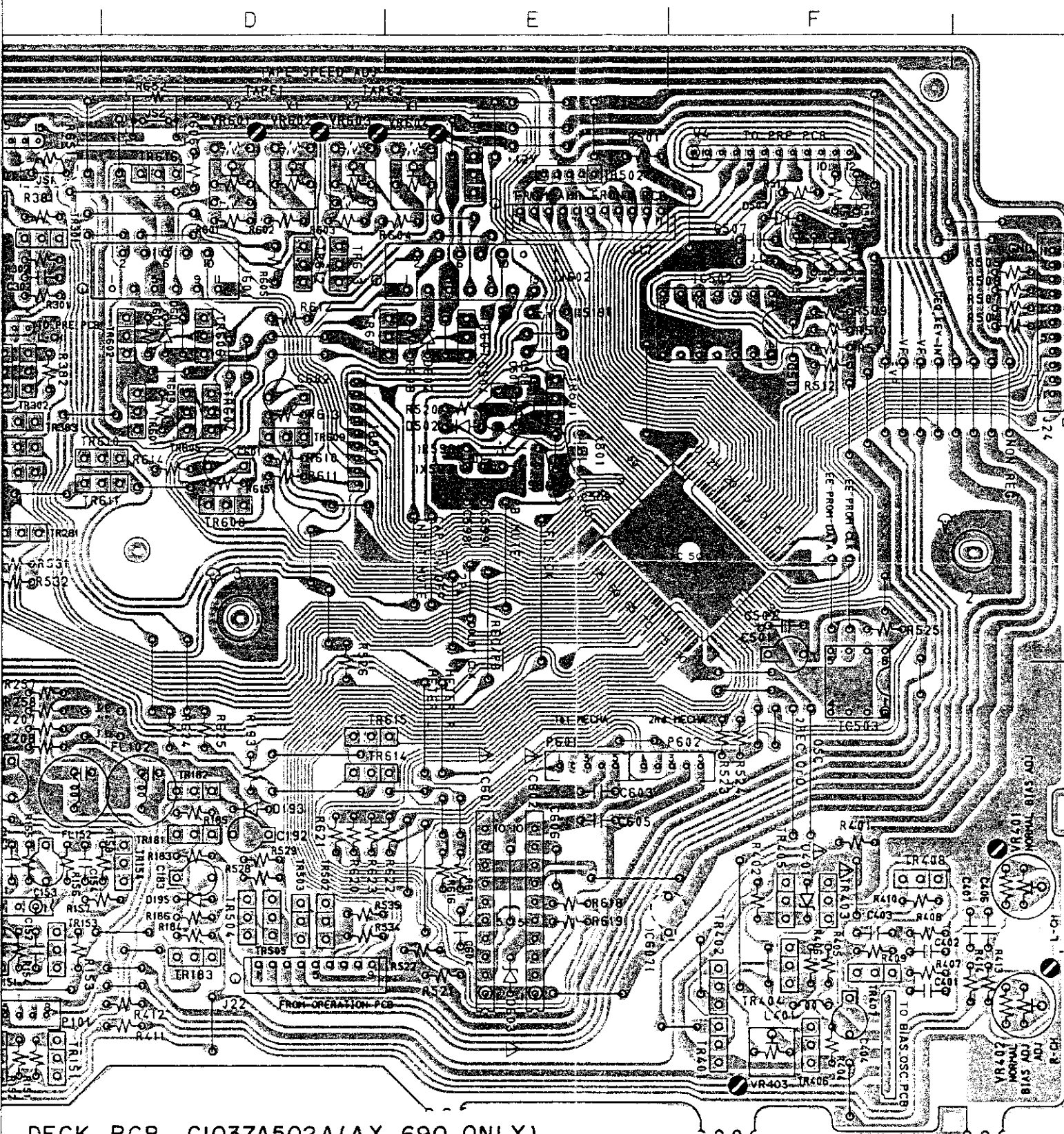
DECK PCB CI037A502A(AX-690 ONLY)
