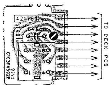
BIAS OSC PCB C1036A502B (AX-590 ONLY)
