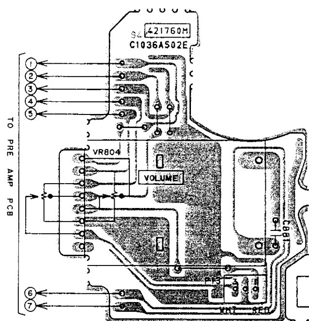
MAIN VOLUME PCB CIO36A502E (AX-590 ONLY)
