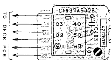
BIAS OSC PCB CI037A502B (AX-690 ONLY)
