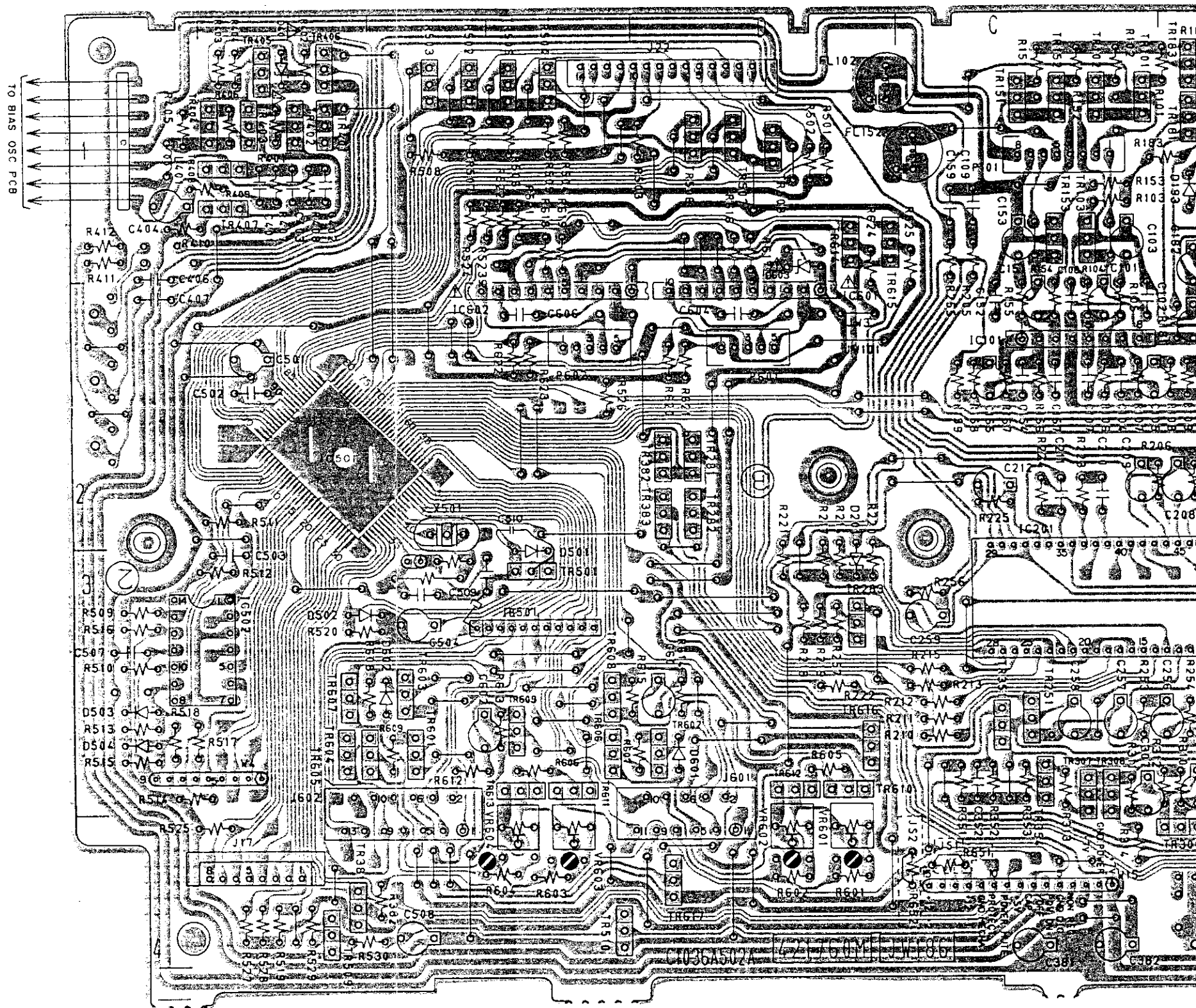
DECK PCB C1036A502A (AX-590 ONLY)
