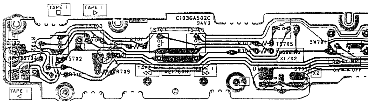
OPERATION PCB C1036A502C
