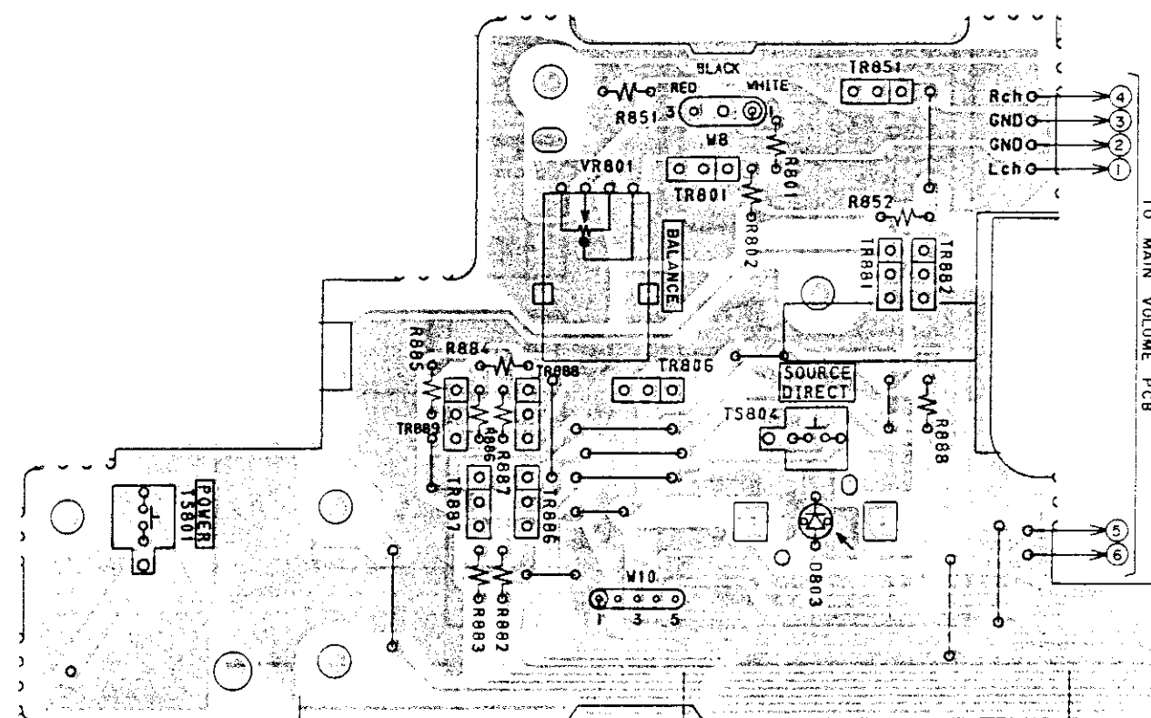
PRE AMP PCB C1037A502E (AX-690 ONLY)
