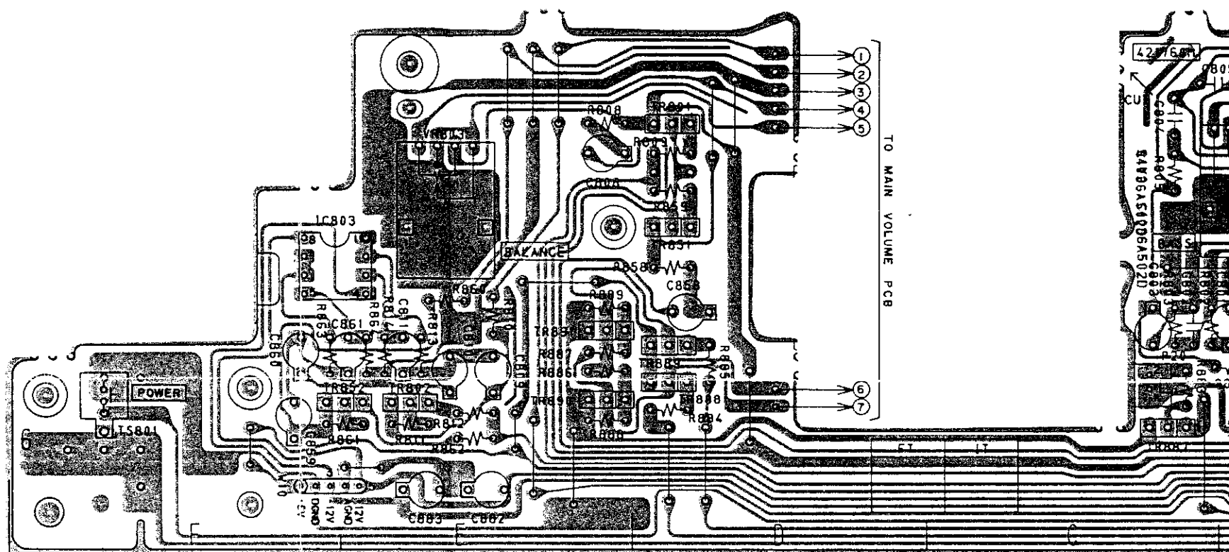
PRE AMP PCB CI036A502D(AX-590 ON
