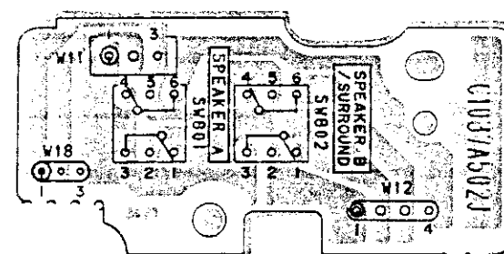
SPEAKER /SURROUND PCB C1037A502J (AX-690 ONLY)
