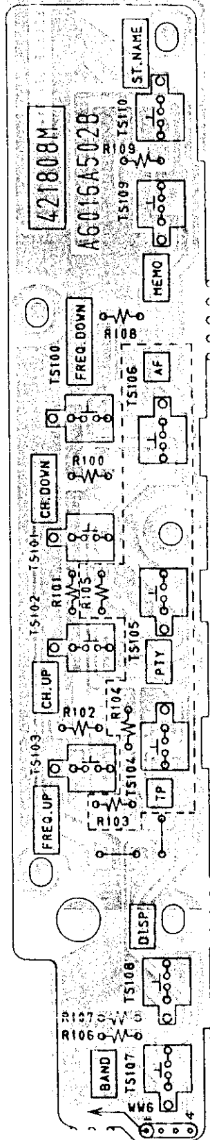
OPERATION PCB A6016A502B(TC-590 ONLY)
