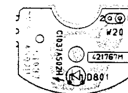
VOLUME LED PCB C1037A502H (AX-690 ONLY)
