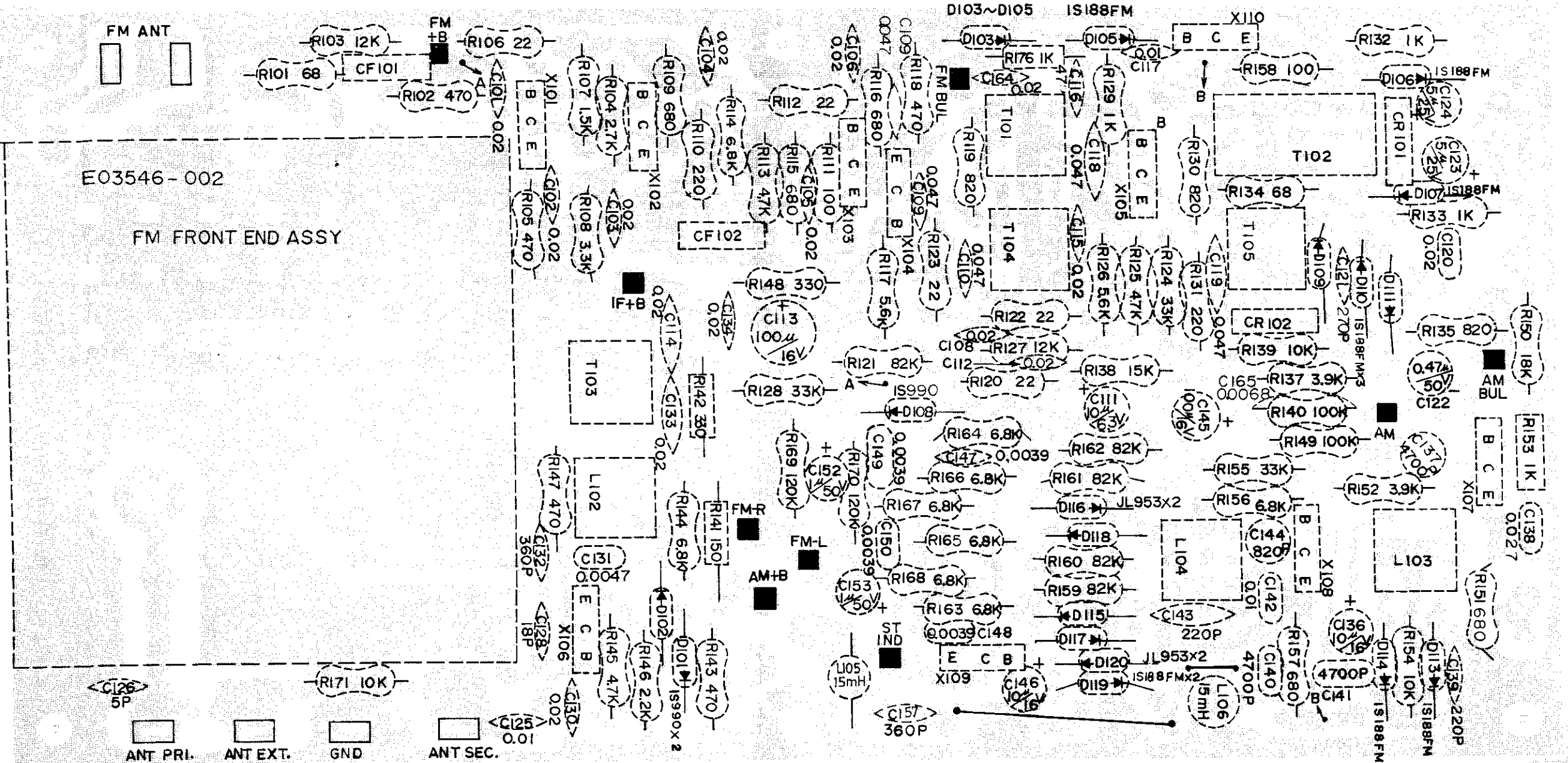
Fig. 13 Bottom View
