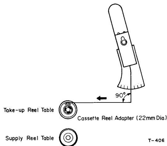
Fig. 5-1 Take-up/Fast Forward Torque Measurement
