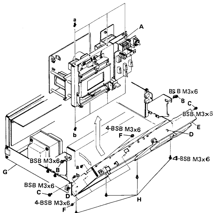
Fig. 4-2 Tape Transport Chassis Removal
