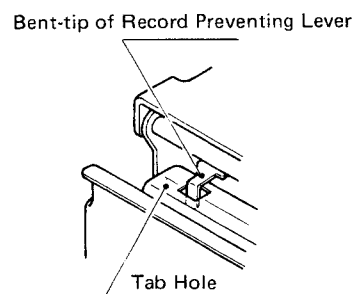
Fig. 5-15 Record Protection Tab Location
