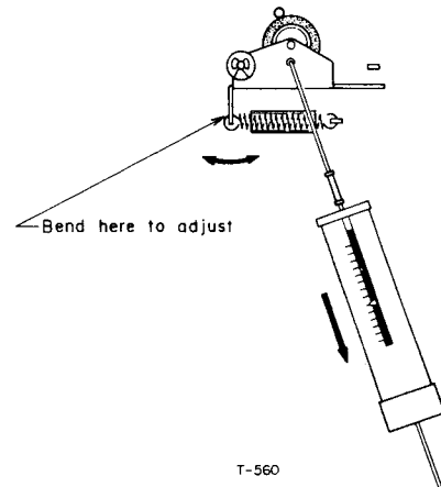
Fig. 5-4 Pinch Roller Pressure Measurement
