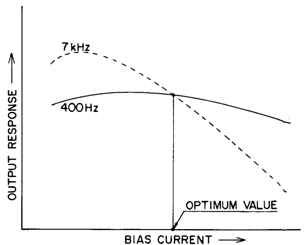
Fig. 6-13 Bias Adjustment (CrO 2 & Fe-Cr tape)
