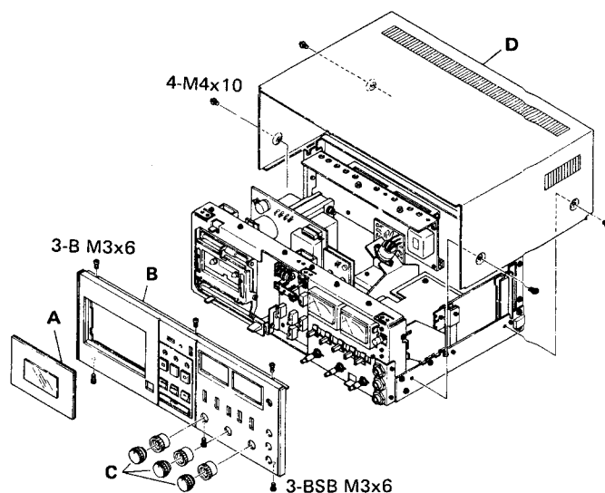
Fig. 4-1 Case/Front Panel Removal
