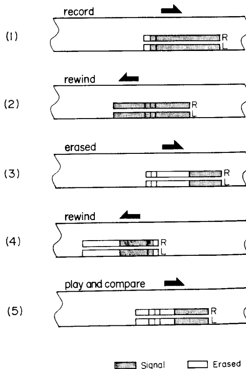
Fig. 6-19 Erase Efficiency Check Procedure
