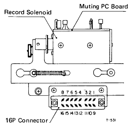
Fig. 6-2 DC Voltage Adjustment
