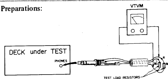
Fig. 6-8 Connection
