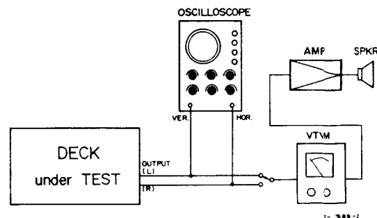
Fig. 6-3 Connection
