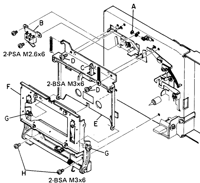
Fig. 4-5 Cassette Holder Removal
