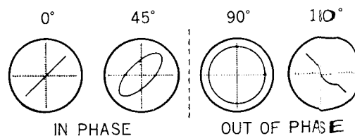
Fig. 6-5 Confirming Phase Relationship
