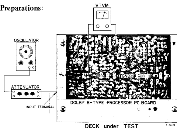
Fig. 6-9 Connection
