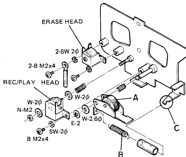
Fig. 4-3 Heads/Pinch Roller Replacement
