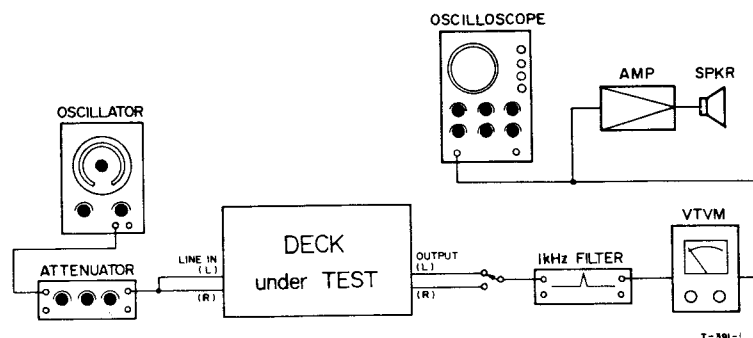
Fig. 6-18 Connection
