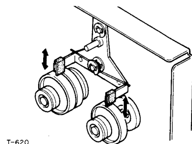
Fig. 5-6 Brake Tension Adjustment
