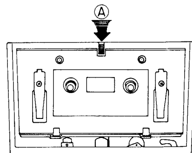
Fig. 5-5 Switch Arm Location
