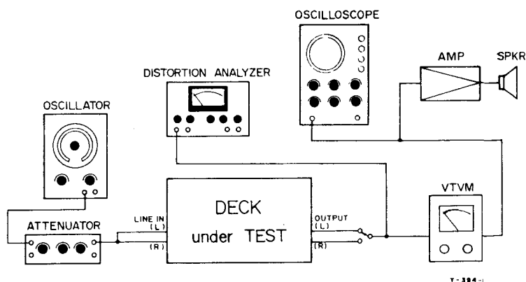
Fig. 6-15 Connection
