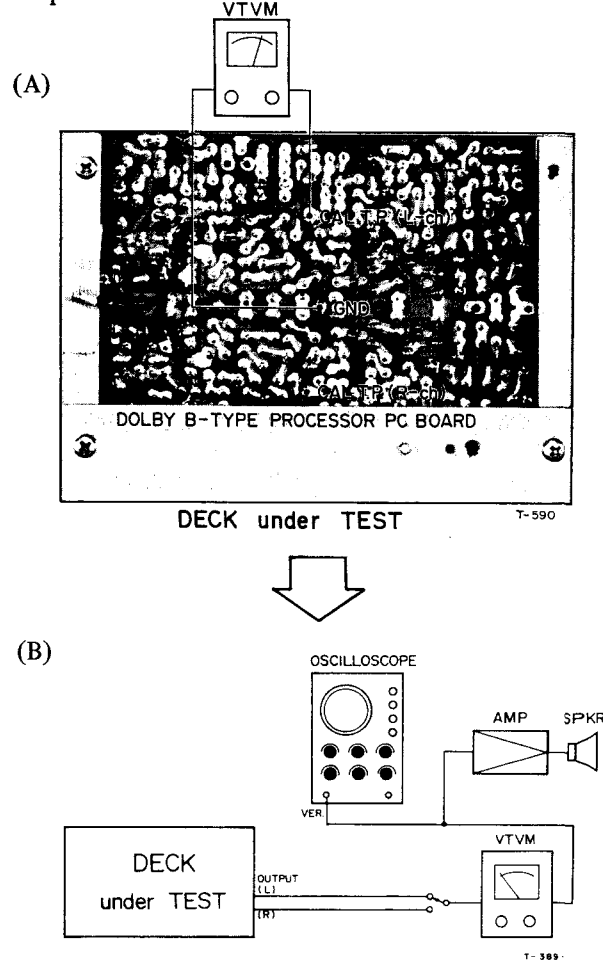
Fig. 6-6 Connection
