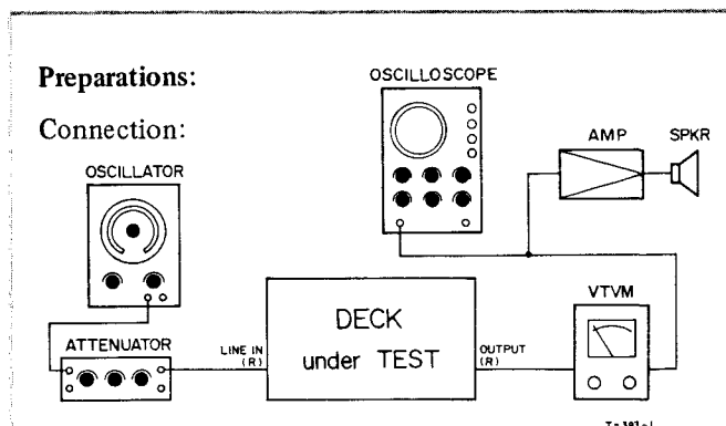
Fig. 6-22 Connection
