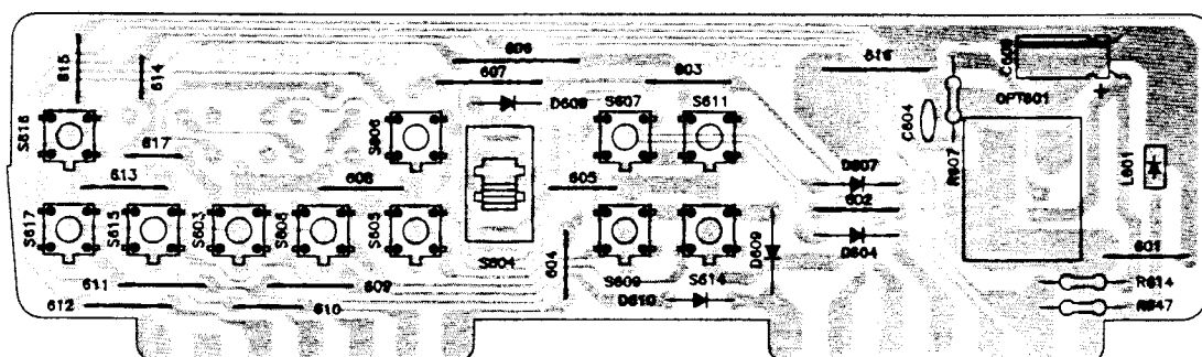
(BOTTOM VIEW)
