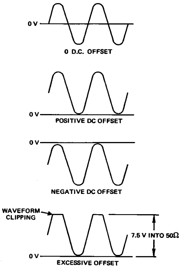
Figure 2-2 - DC Offset Control
