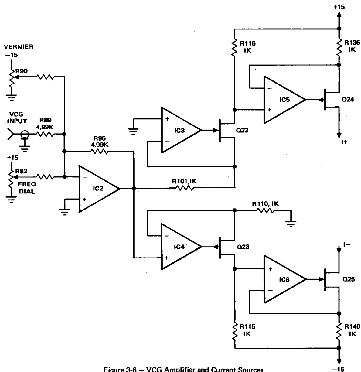
Figure 3-6 – VCG Amplifier and Current Sources
