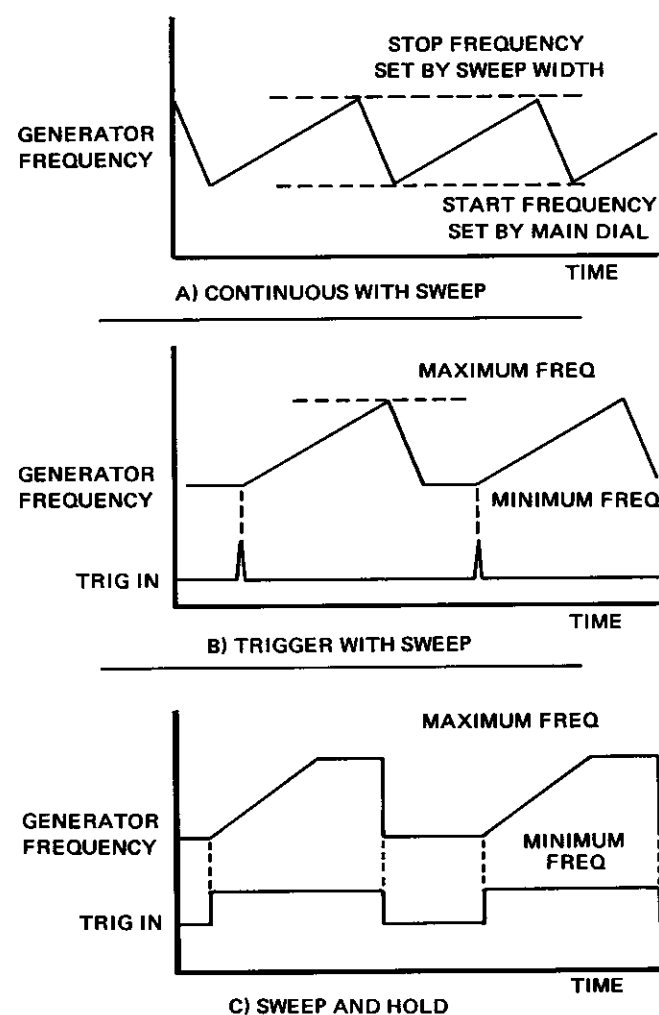
Figure 2-6 - Generator Sweep Modes
