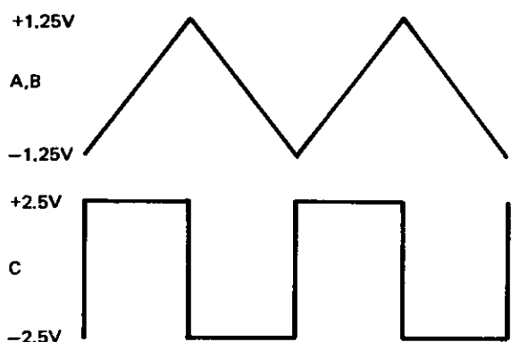
Figure 3-2 - Simplified Timing Diagram
