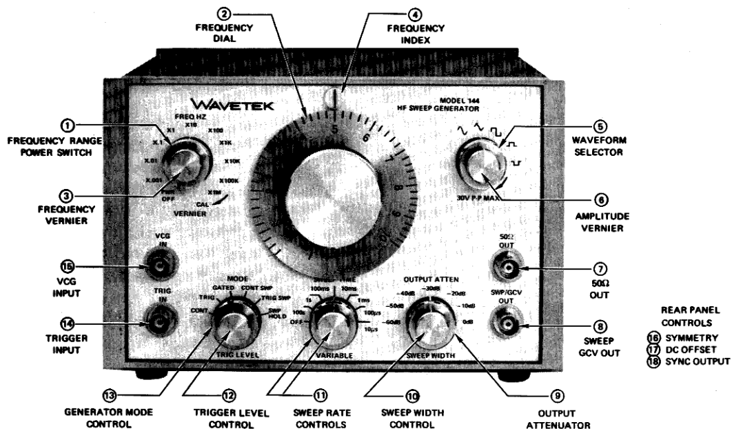
Figure 2-1 - Operating Controls
