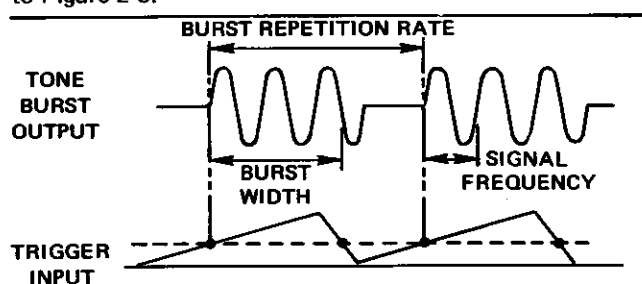
Figure 2-5 - Tone Burst Controls
