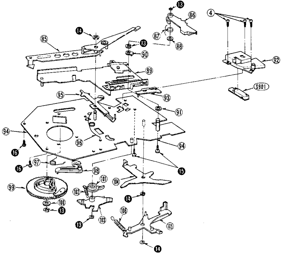
AUTOMATIC MECHANISM ASS'Y
