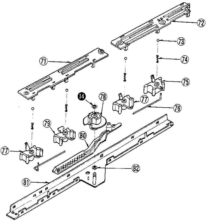
AUTOMATIC MECHANISM ASS'Y
