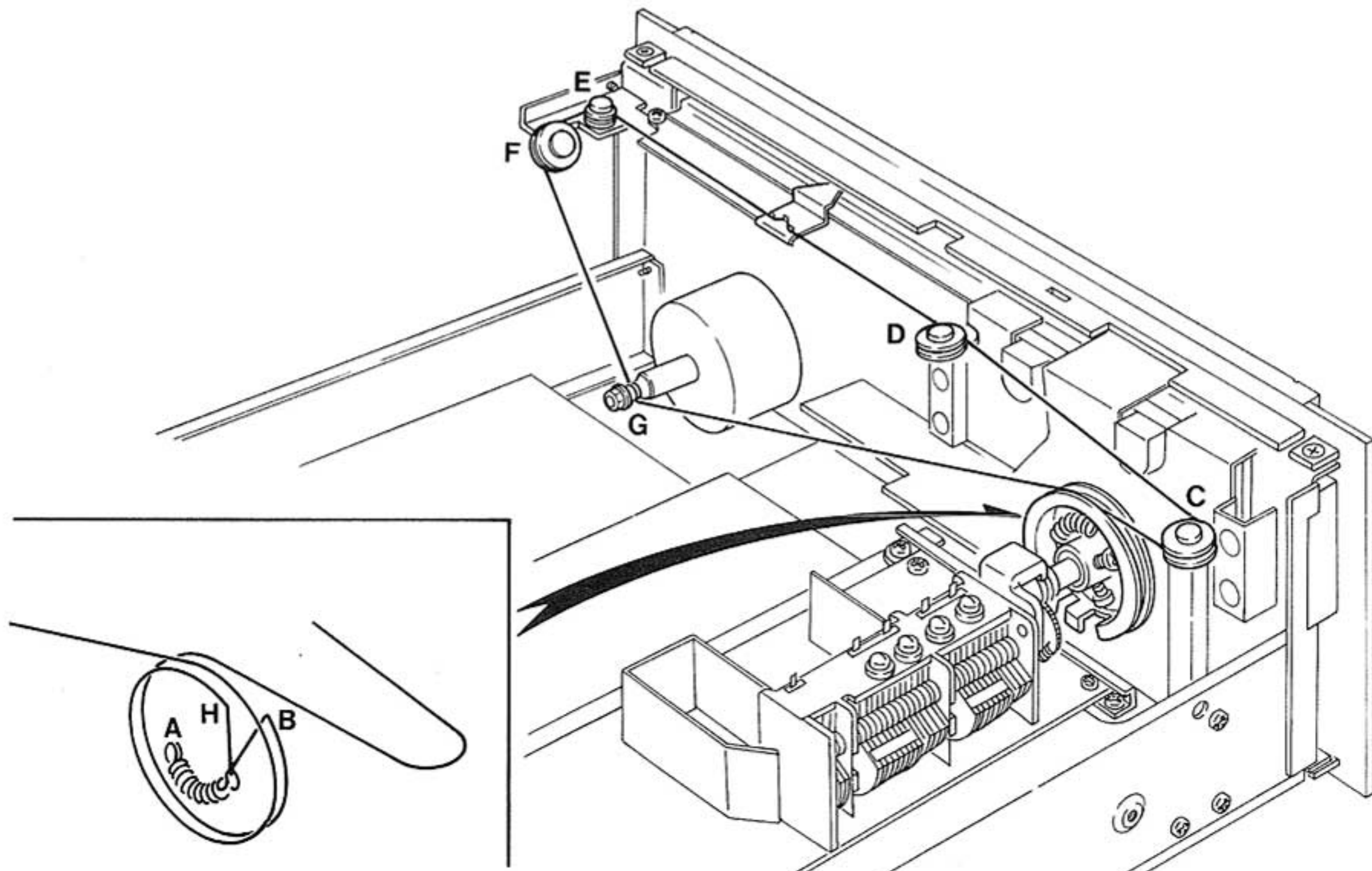
Figure 1. Dial Stringing
