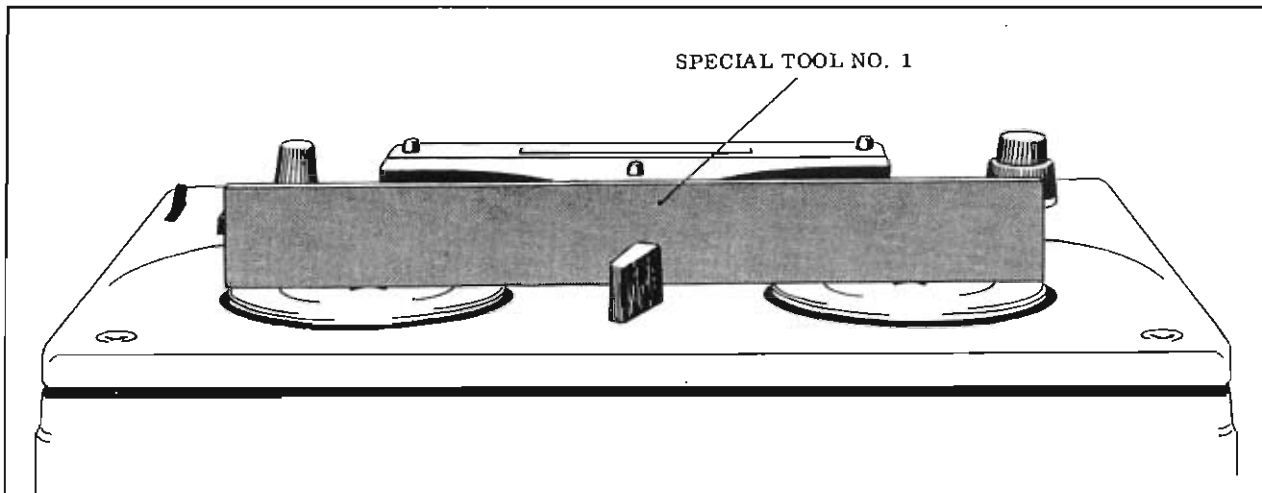
Fig. 4.11 Horizontal adjustment of turntables
