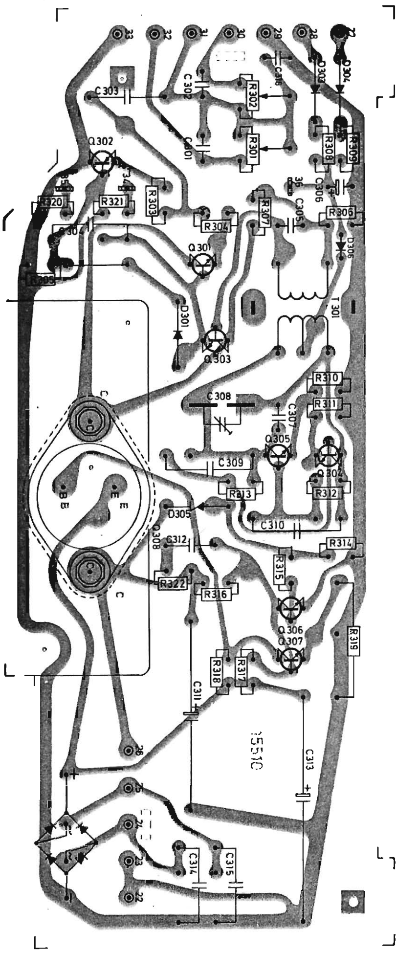
Detector and oscillator board, printed side.
