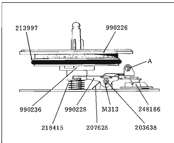
Fig. 4.14 Supply Turntable
