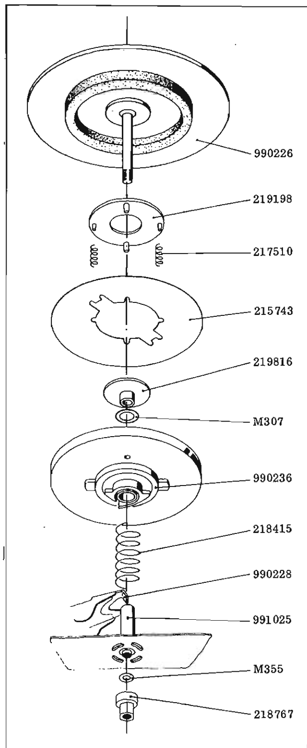
Fig. 4.6 Supply turntable
