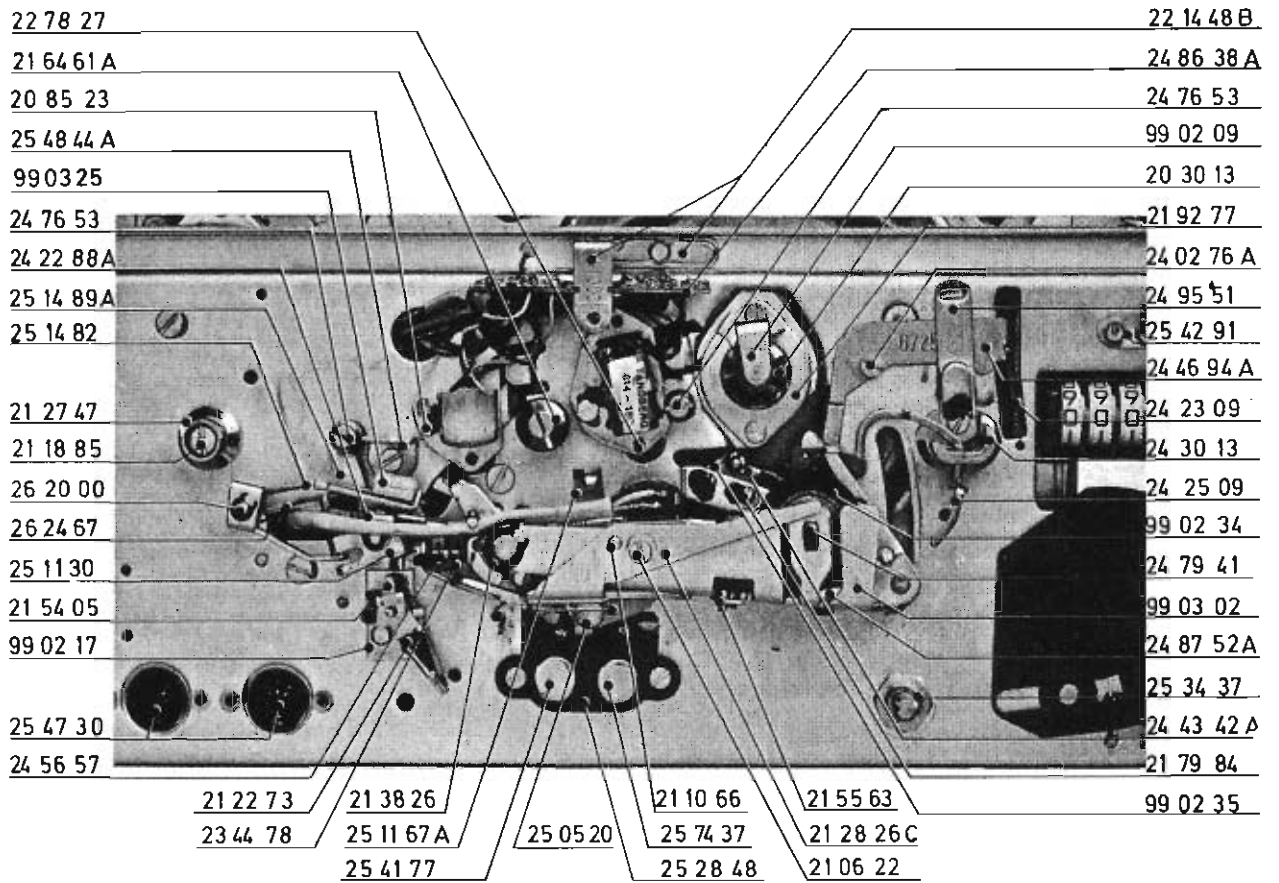
Fig. 4.4 Tape path
