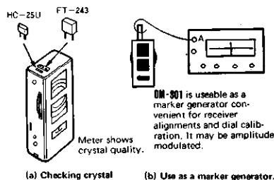
Figure 7 — Use as a Crystal-Controlled Signal Generator.
