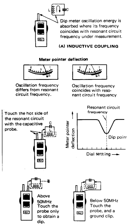
Figure 1. Dip Meter Operation
