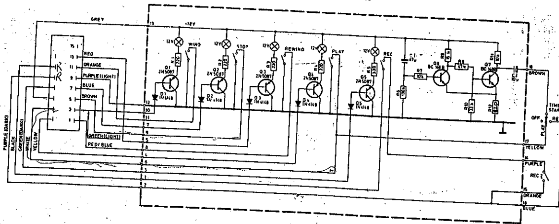
FIG. 6. REMOTE CONTROL
