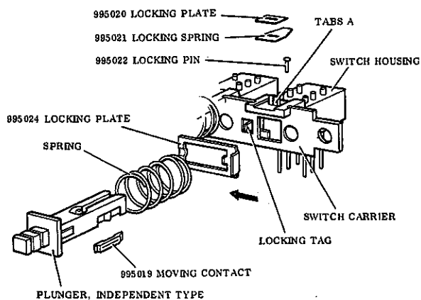
Fig. 7 Switches
