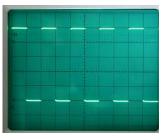
C2110 undercompensate
