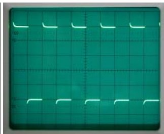
C2108 overcompensate
