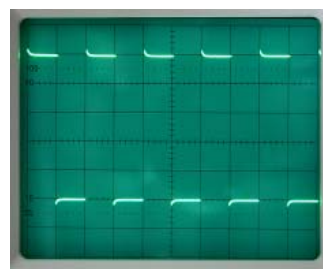
C2011 overcompensate
