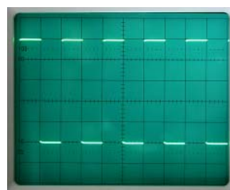
C2011 undercompensate
