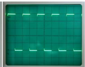
C2010 undercompensate
