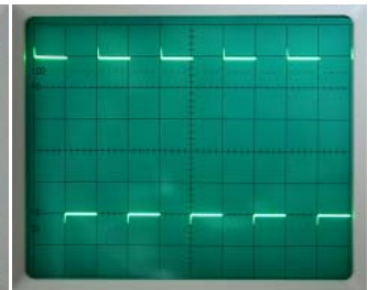
C2010 overcompensate
