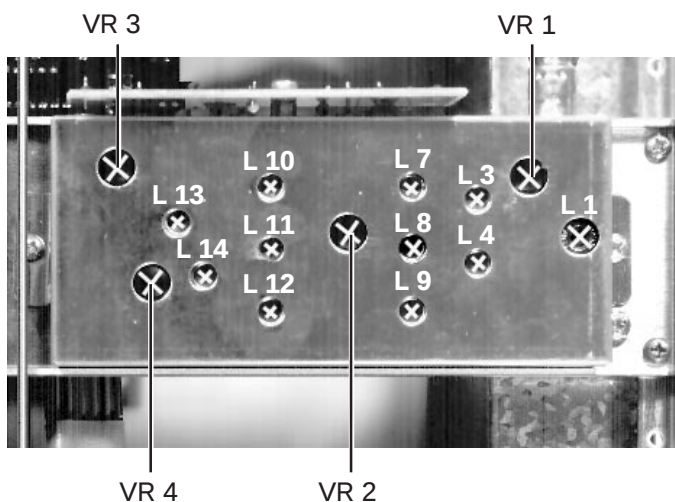
PIC 5 IF-Amp Board
