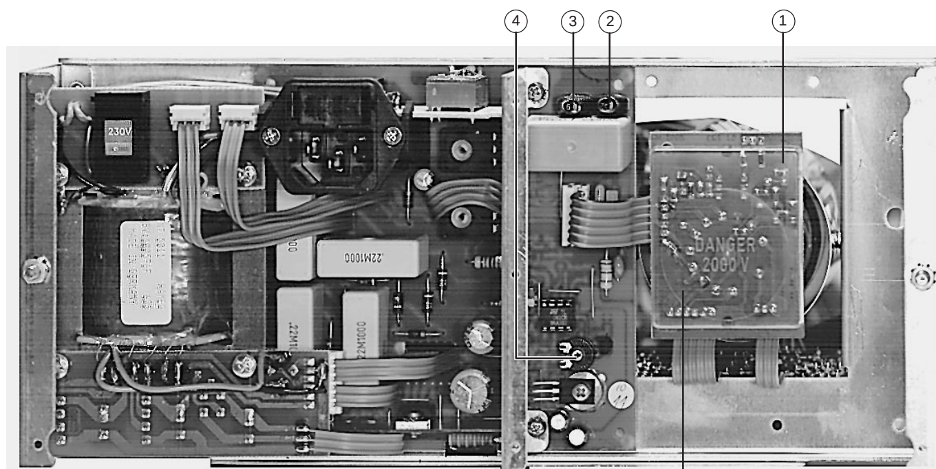
PIC 1. PS-Board
