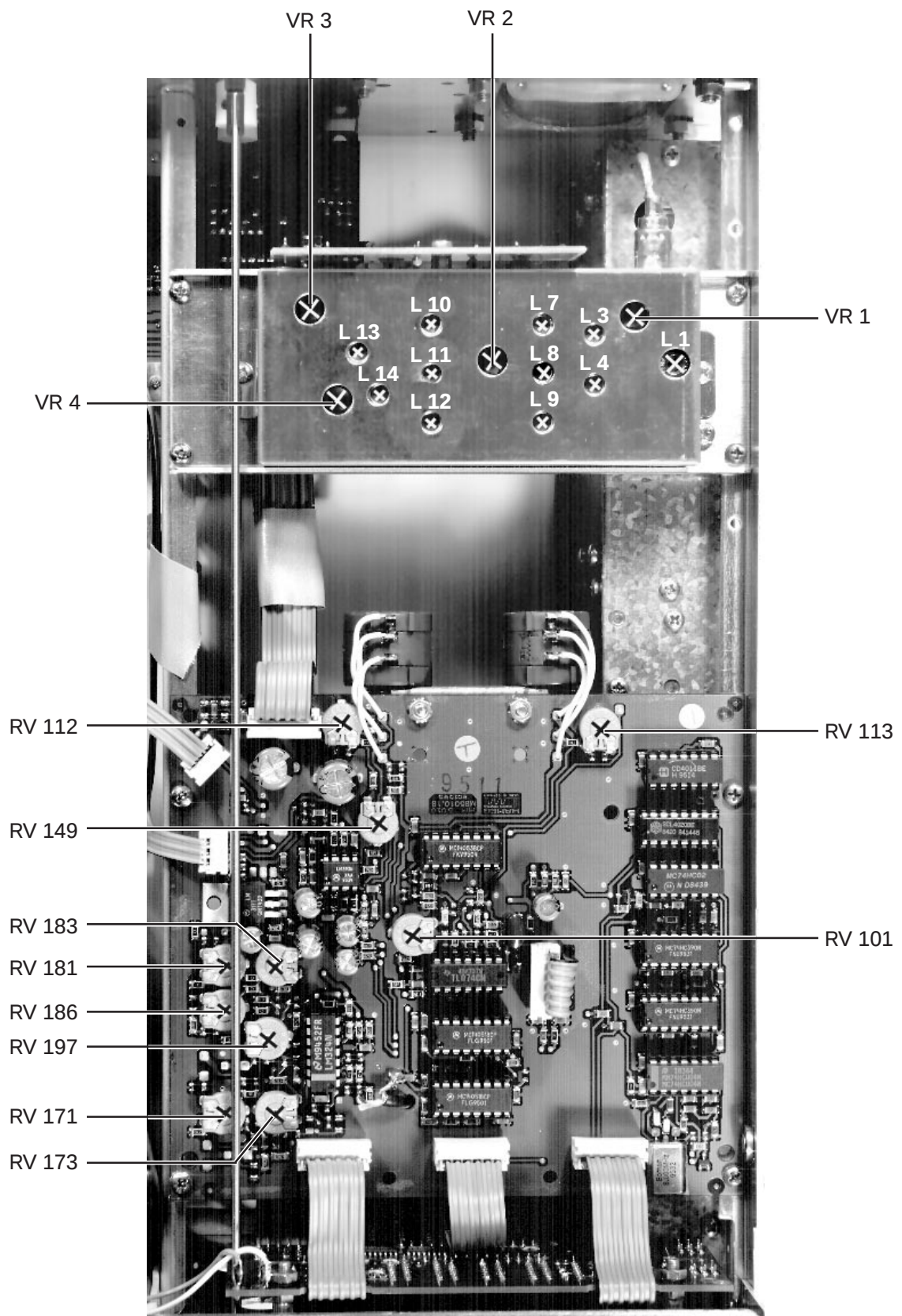
PIC 3 - Main-Board
