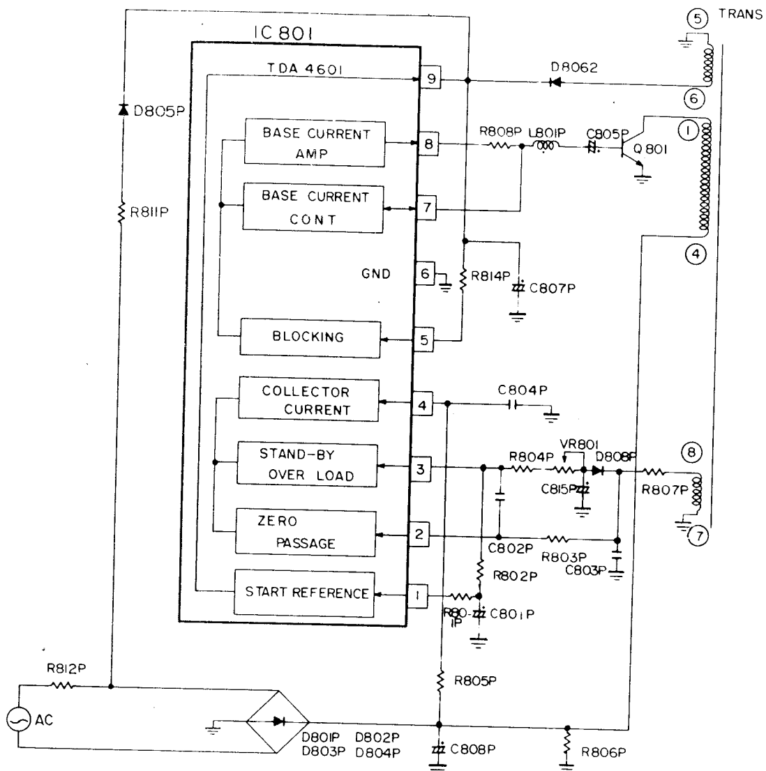
Figure 16. Schematic Diagram of IC801 (TDA4601)
