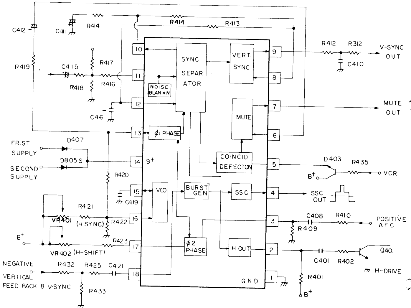
Figure 13. Schematic Diagram of IC401
