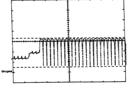
X-42b 2V/div 100µs/div 5,6V
