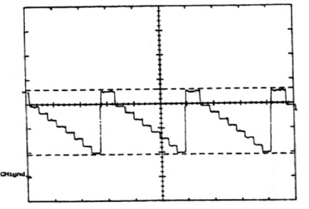
X-40 50V/div 10µs/div 134V
