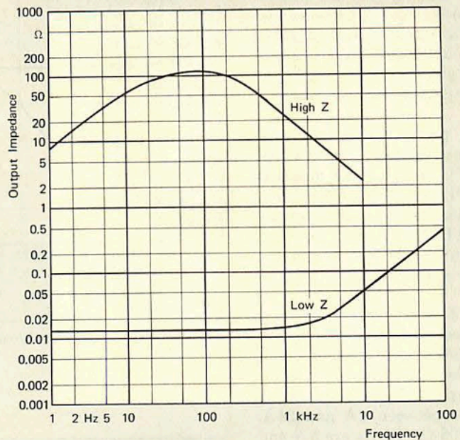
Fig. 2. Typical output impedance curves for Type 2707
