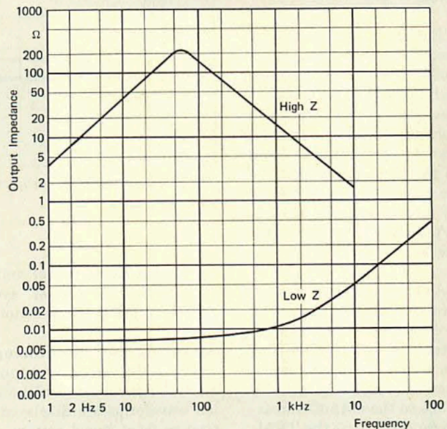
Fig. 3. Typical output impedance curves for Type 2708
