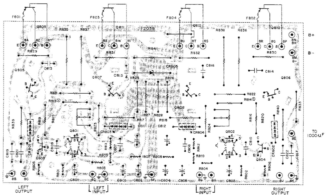
BOARD VIEWED FROM COMPONENT SIDE
