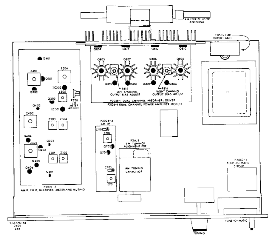
(250-T) CHASSIS LAYOUT
