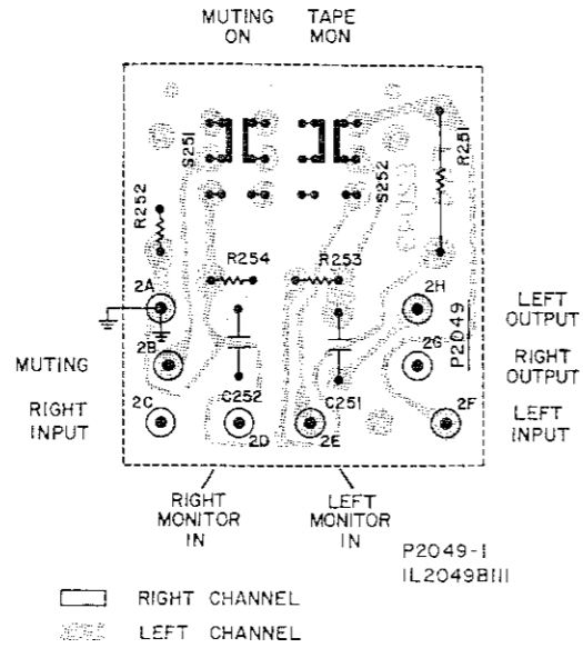
BOARD VIEWED FROM COMPONENT SIDE
