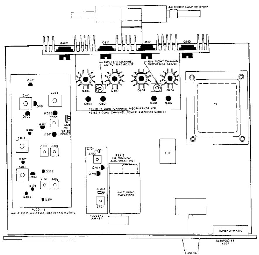
(400-T) CHASSIS LAYOUT
