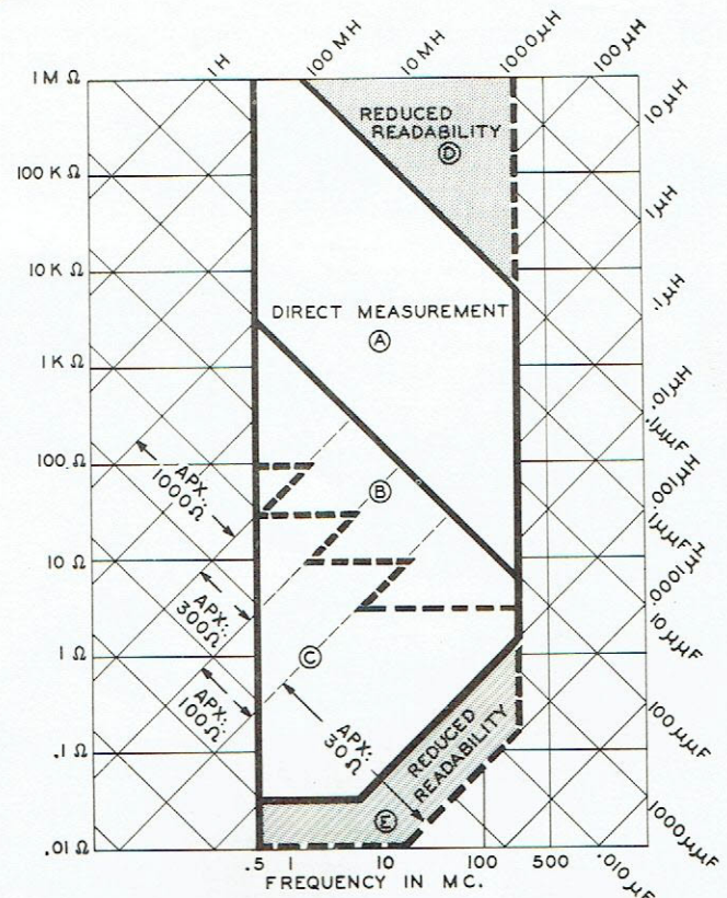
Figure 3 Inductance measurement range
