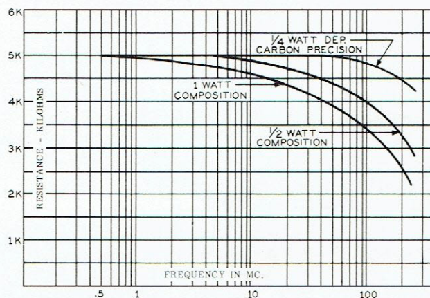
Figure 2 Typical resistor measurements
