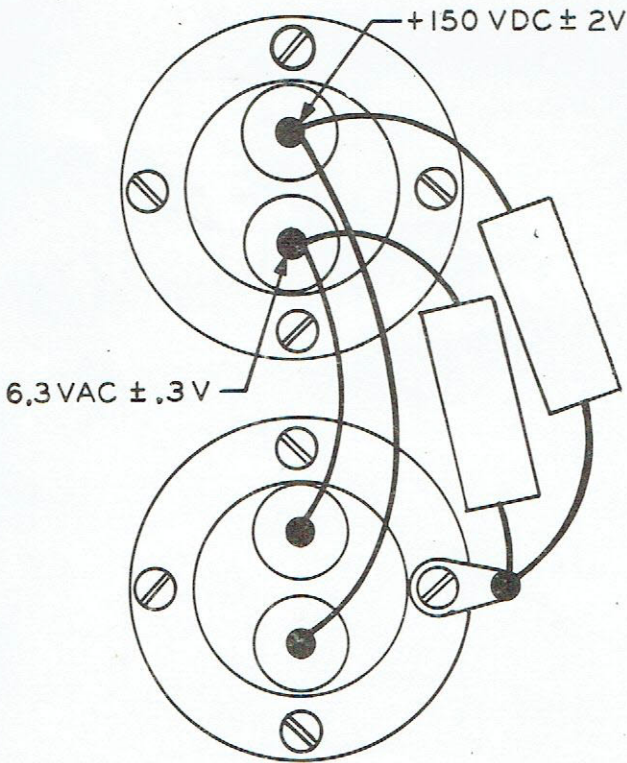
TOP OF OSCILLATOR CASTING
