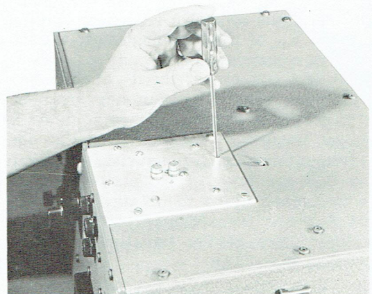
Figure 13 Adjustment of bridge trimmer
