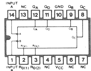
SN7493N 4-bit binary counter
