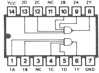
SN7420N Dual 4-input NAND gate
