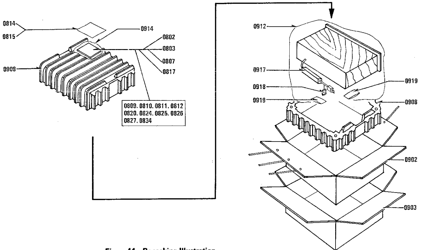
Figure 11. Repacking Illustration
