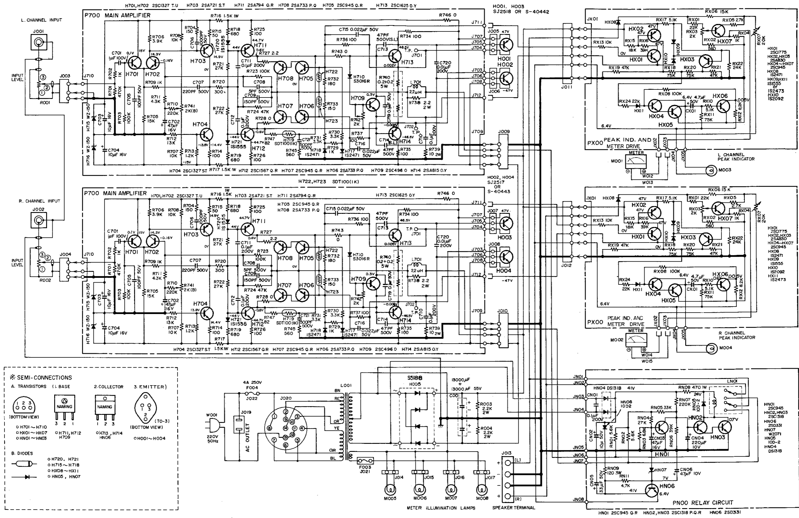
Figure 14. Schematic Diagram
