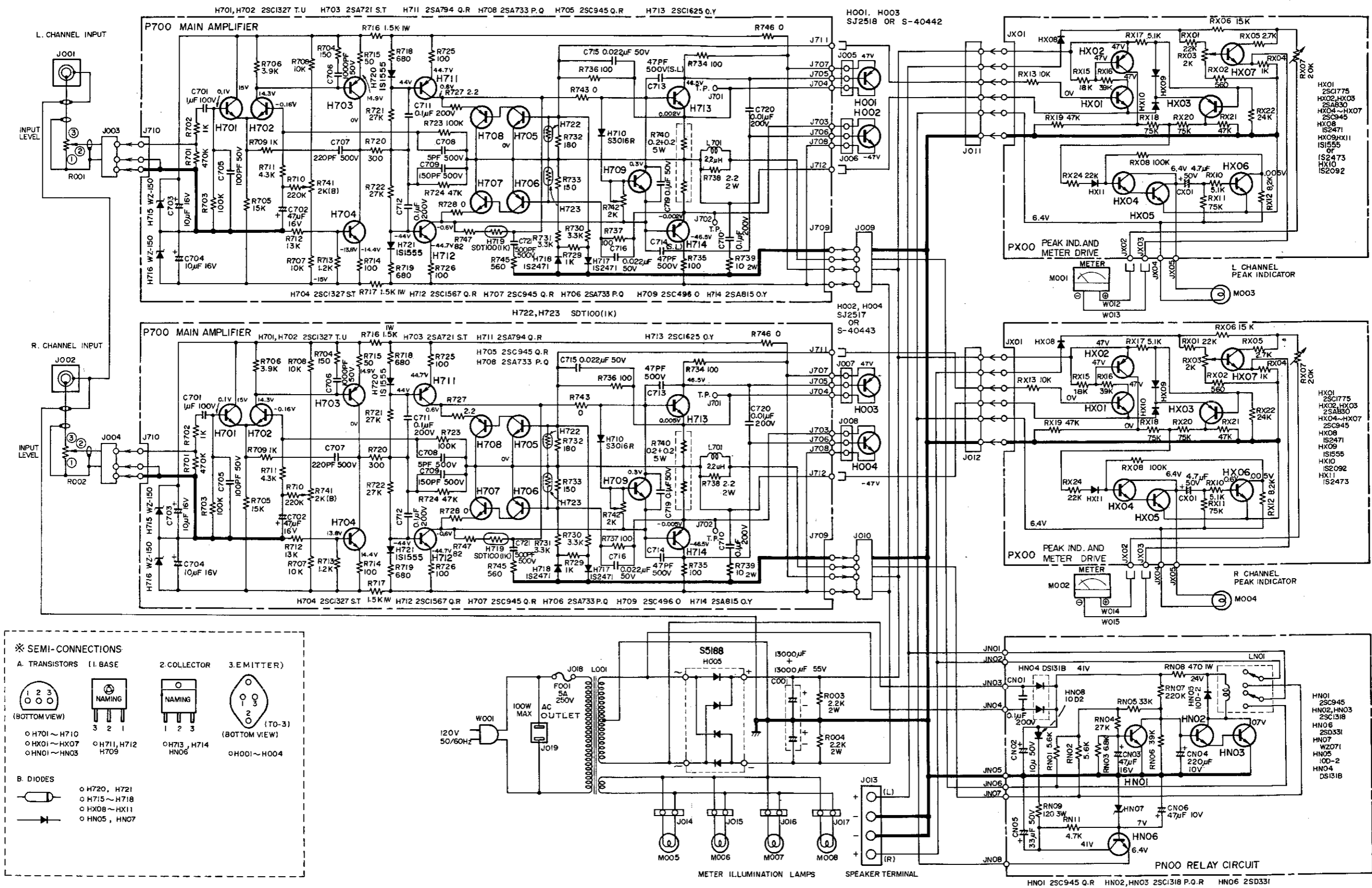
Model 140 NOTE: This schematic diagram applies to units manufactured for the U.S.A. market.
