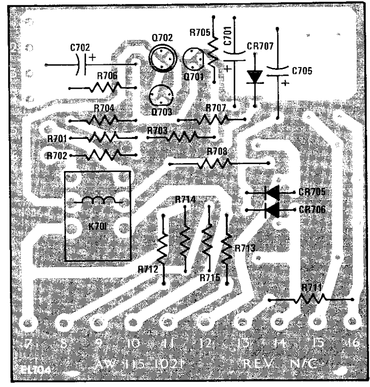
Figure 19. Relay Board – A8 Component Assembly Diagram
