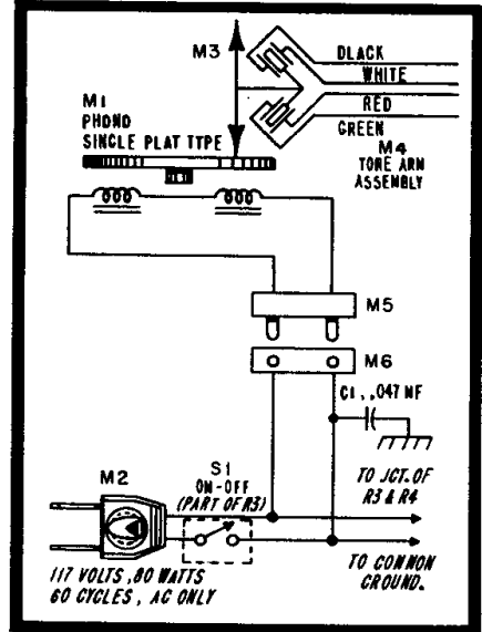
AC INPUT CIRCUIT FOR 2E1 CHASSIS
