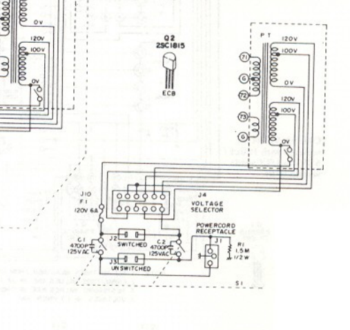
AC Input Circuit of Units for US/Canada.
