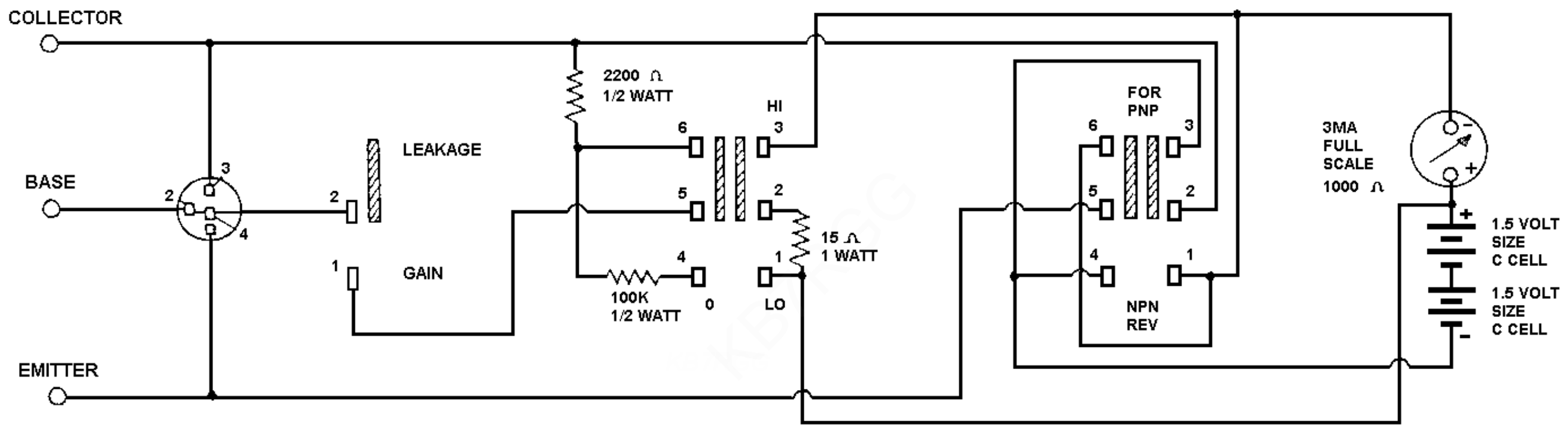
SCHMATIC OF THE HEATHKIT TM TRANSISTOR-DIODE CHECKER MODEL IT-27
