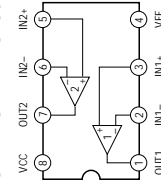
CVM BOARD : IC1801 M5216P
