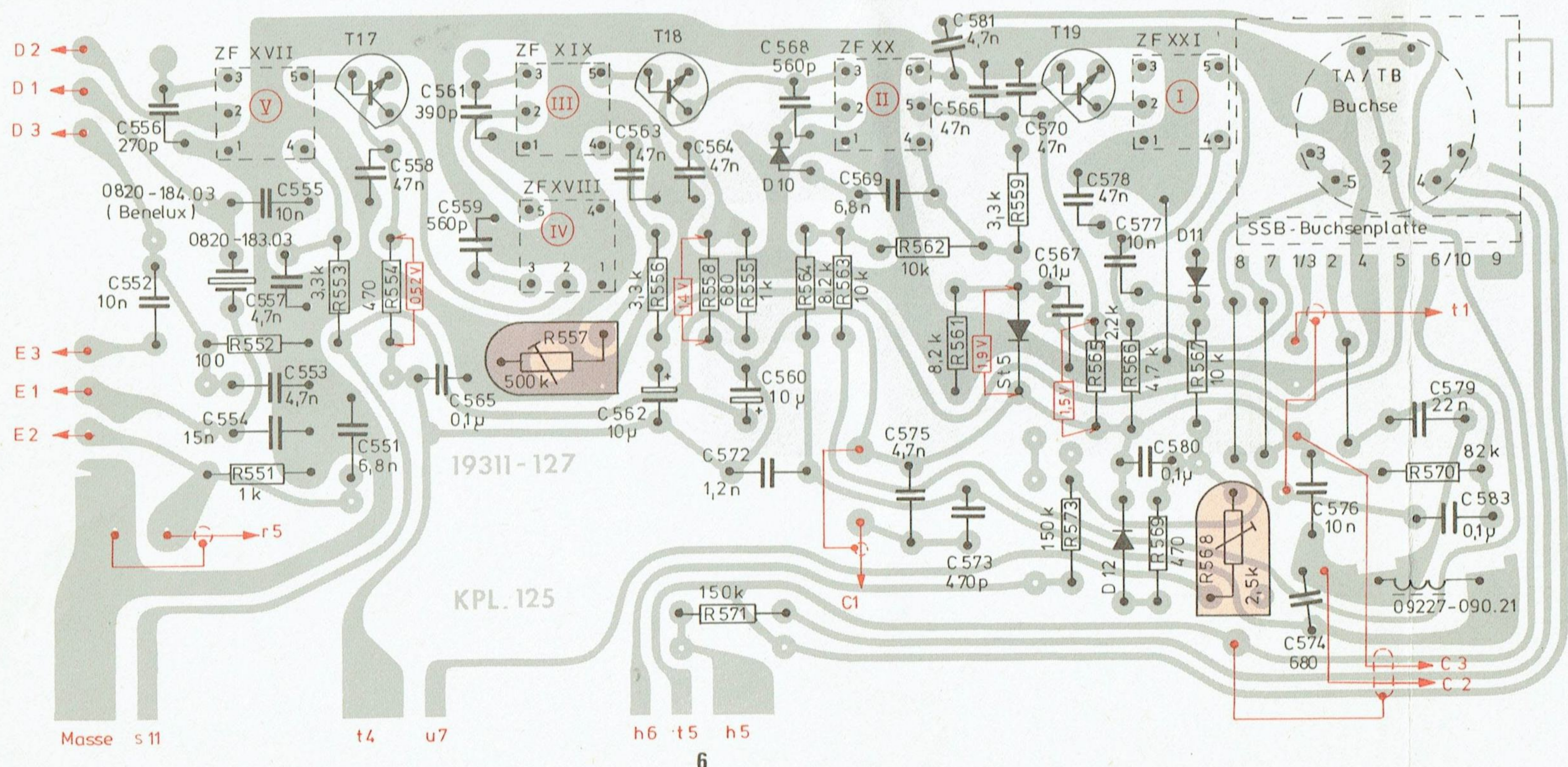
AM-ZF-Platte, Lötseite AM-IF-PRINTED BOARD, SOLDER SIDE PLAQUE AM-FI, COTE SOUDURES PIASTRA AM-FI, LATO SALDATURE
