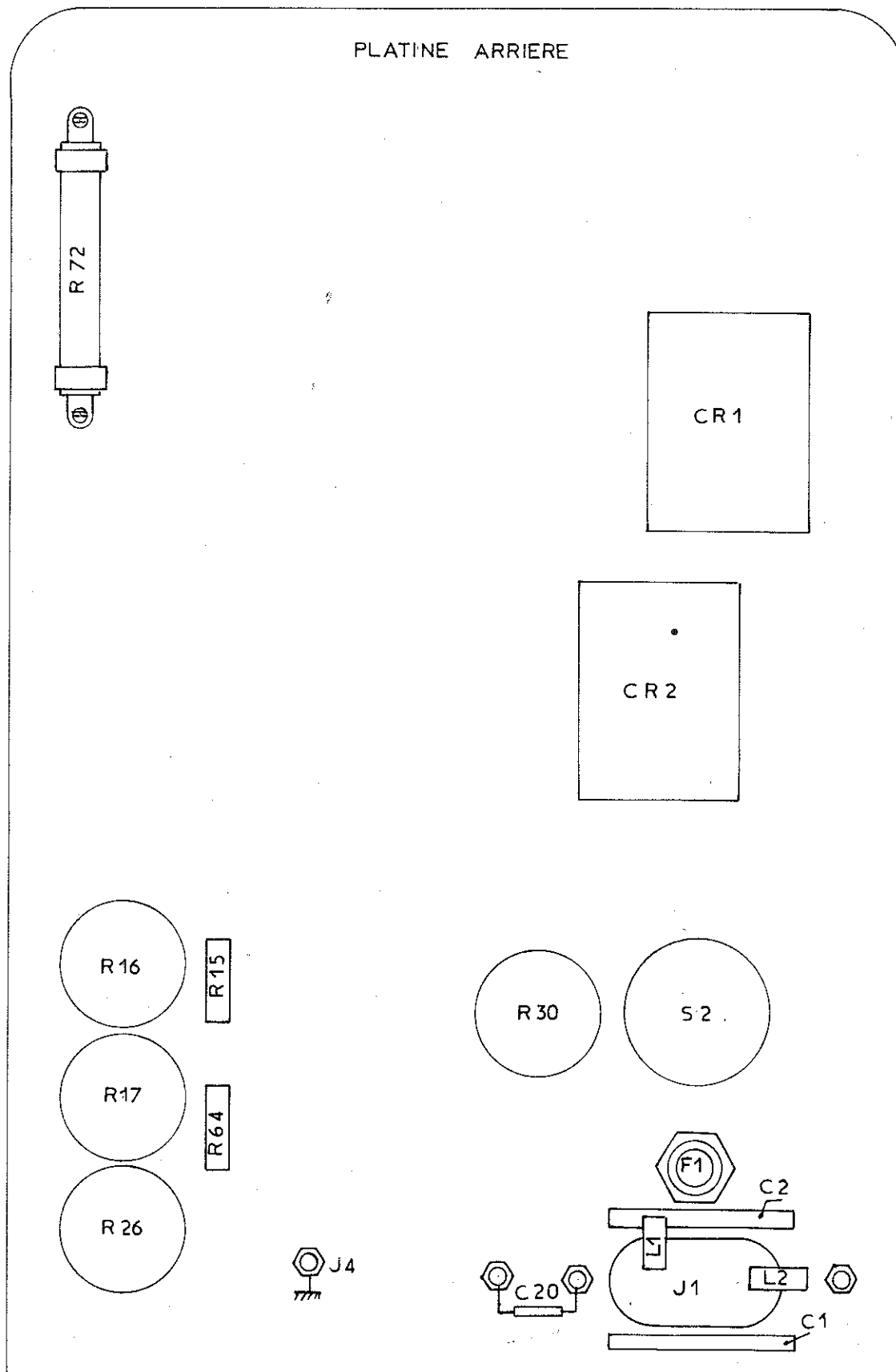
VOLTOHMMETRE ELECTRONIQUE 746A METRIX EMPLACEMENT DE PIECES
