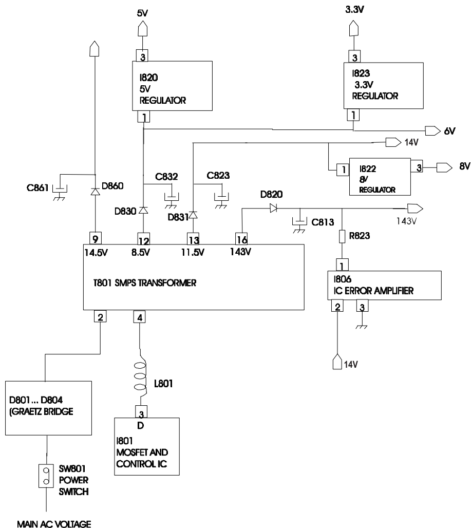
Fig : Power supply operation during TV set normal run
