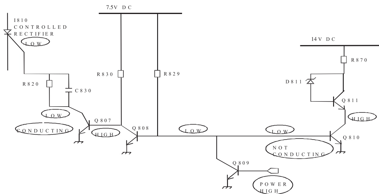
Fig : I501 microcontroller part pin 1 (POWER) effect
