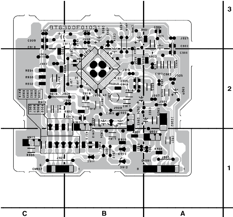
Text CBA Bottom View
