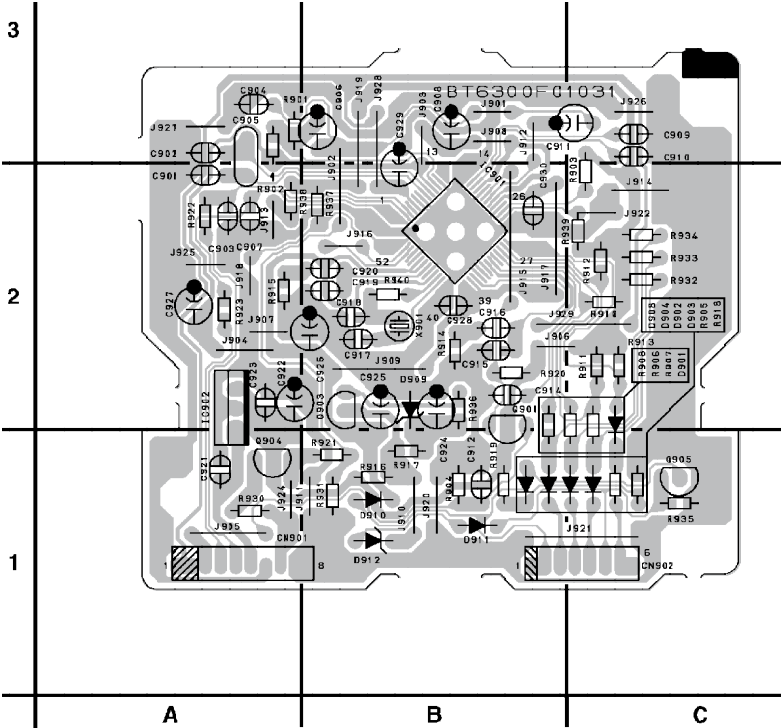
Text CBA Top View
