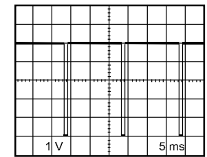
WF18 MAIN 1/4 SCHEMATIC DIAGRAM IC201 PIN 59
