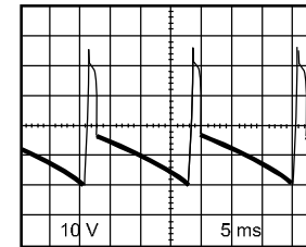
WF13 H.V./POWER SUPPLY 2/2 SCHEMATIC DIAGRAM CN571 PIN 5
