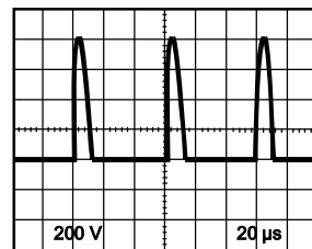
WF12 H.V./POWER SUPPLY 2/2 SCHEMATIC DIAGRAM Q571 COLLECTOR
