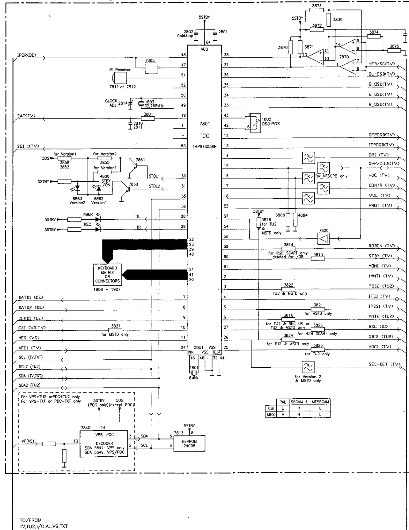
CONTROL PART (CO) Small Signal Board
