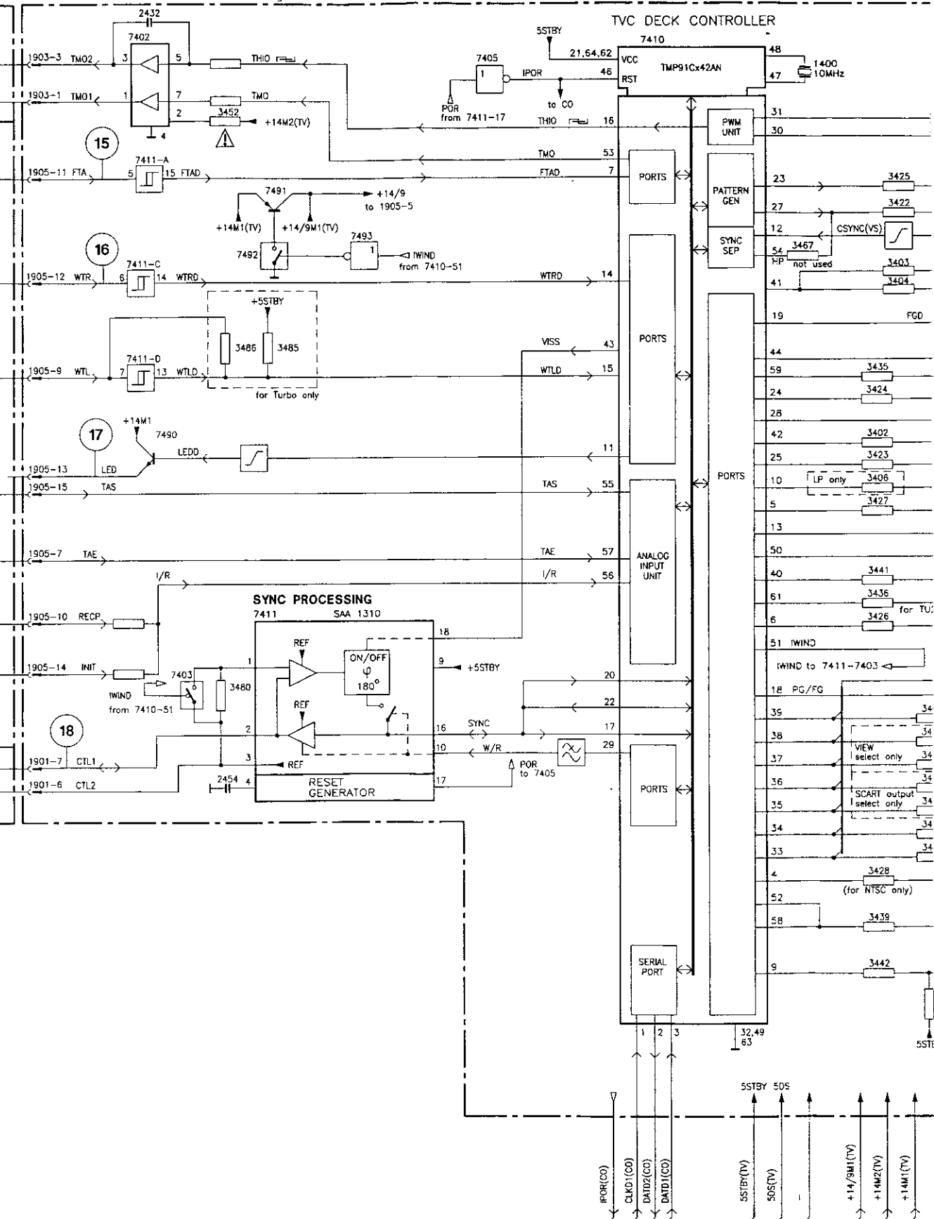
DECK ELECTRONIC (DE) Small Signal Board
