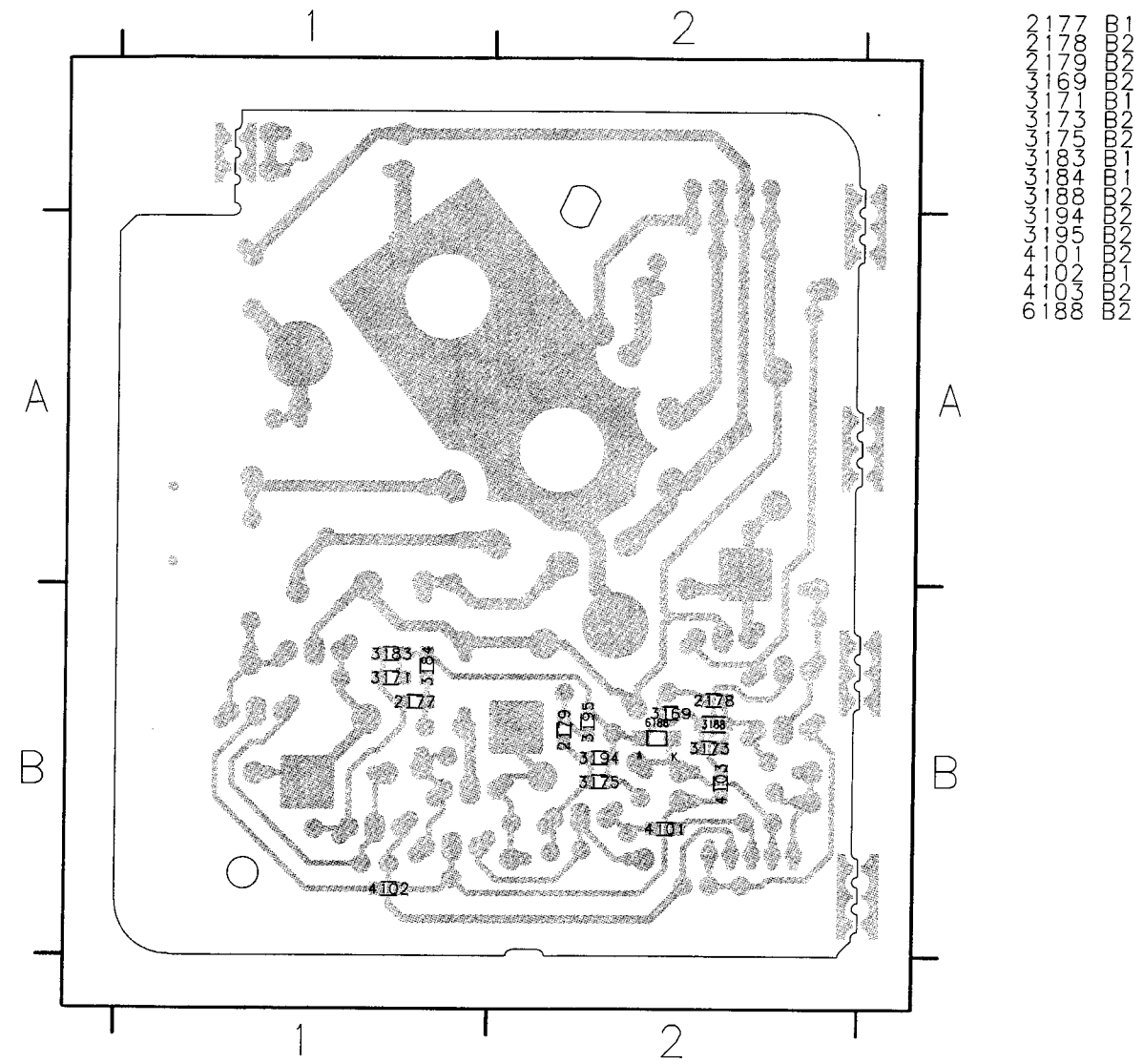
7.27 CRT Panel 14" (PT) LSB1L14 - Solder Side
